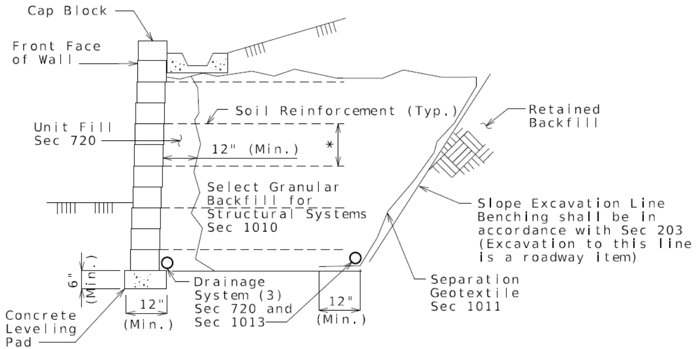
Fig. 751.24.2.23.2 Typical Section Through Generic Drycast Modular Block Wall (DMBW-MSE) System or Wetcast Modular Block Wall (WMBW-MSE) System Small Block Wall
