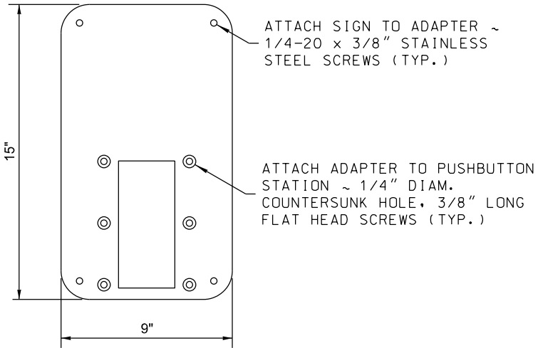
PEDESTRIAN PUSHBUTTON FRAME ADAPTER
