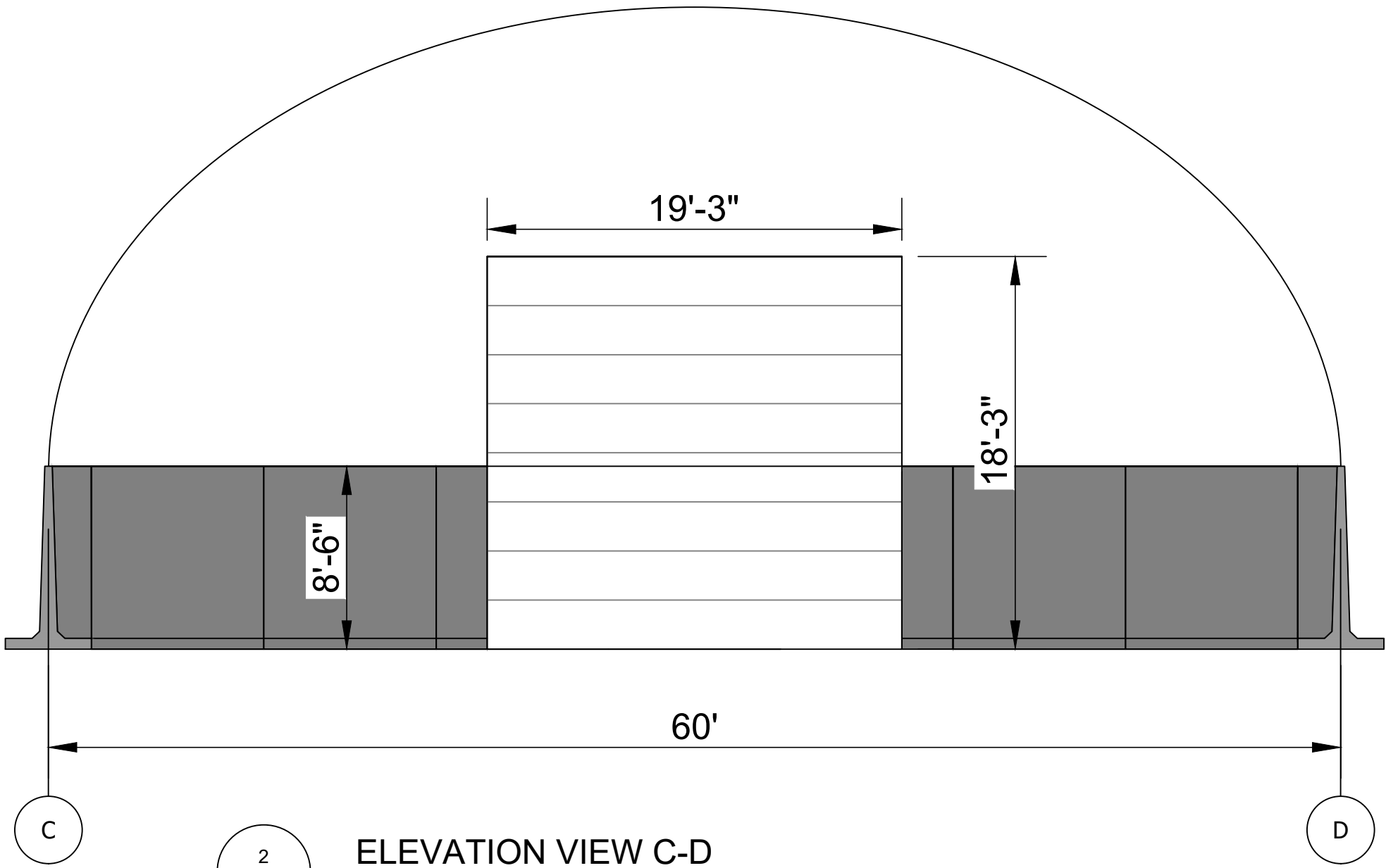
2 ELEVATION VIEW C-D NO SCALE
