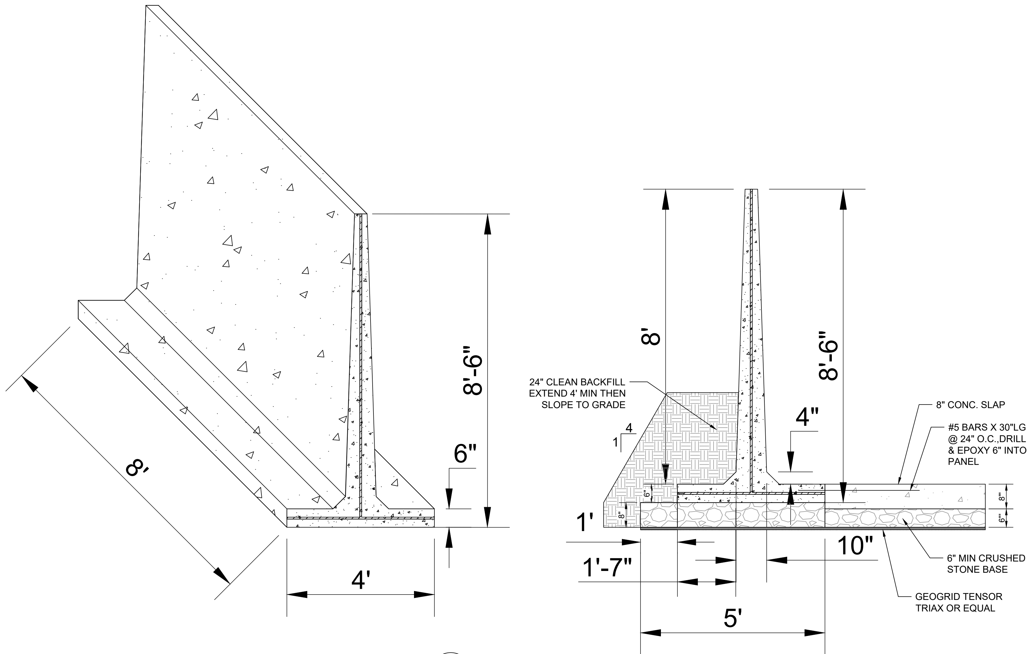
4 PRECAST T WAL DETAILS NO SCALE
