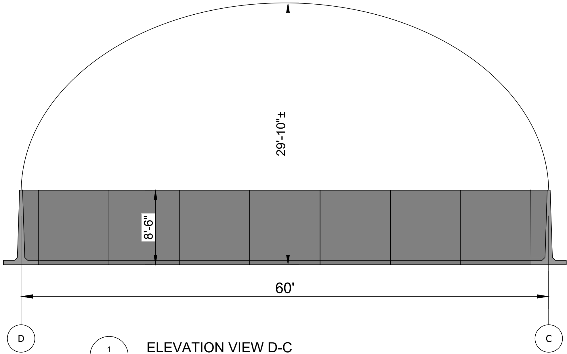
1 ELEVATION VIEW D-C NO SCALE
