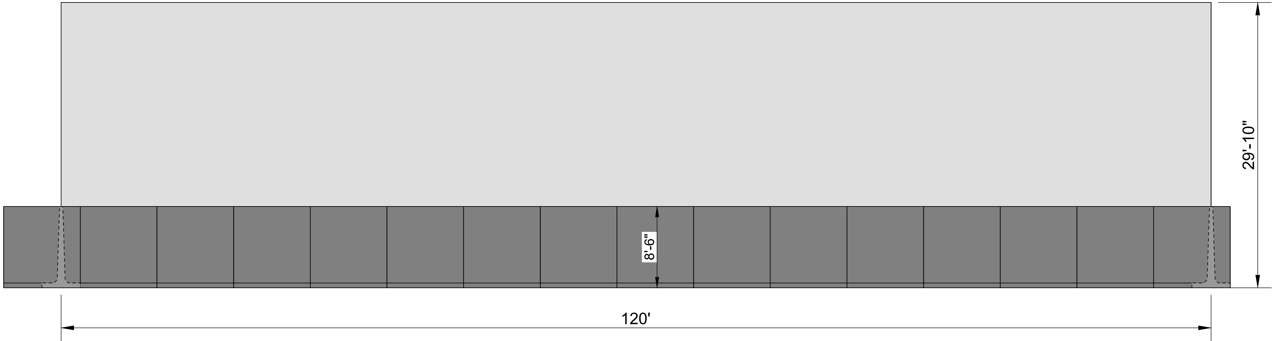
3 ELEVATION VIEW A-B NO SCALE
