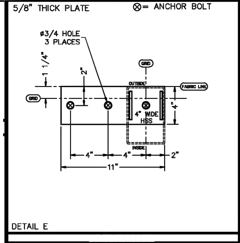
8 SADDLE BRACKET DETAILS NO SCALE
