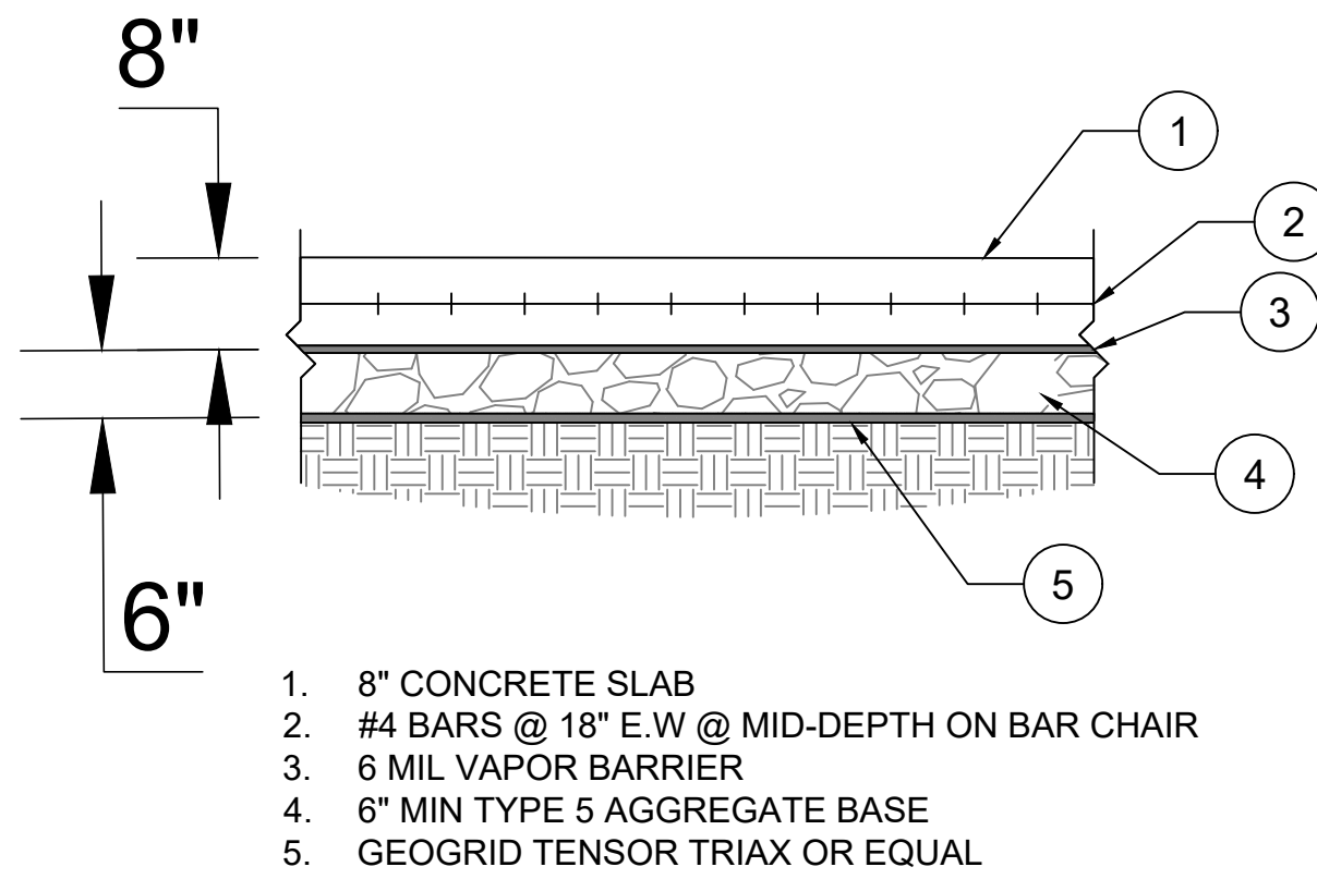
7 CONCRETE SLAB DETAIL NO SCALE
