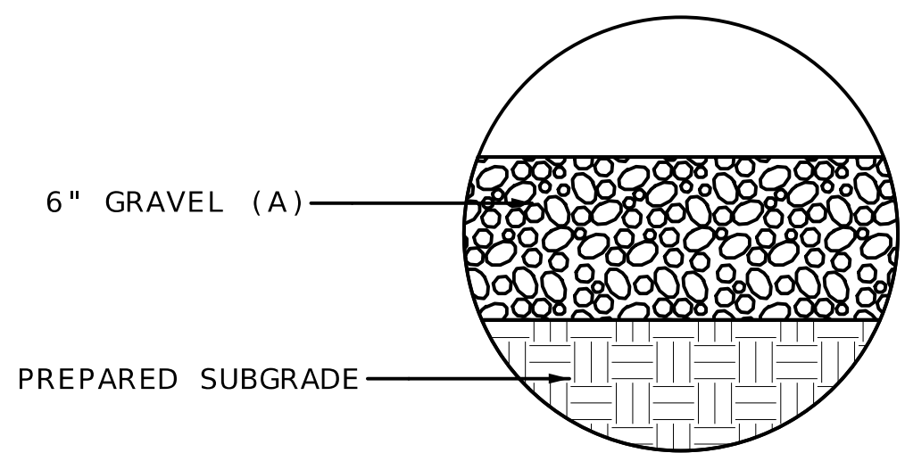
GRAVEL AREAS
