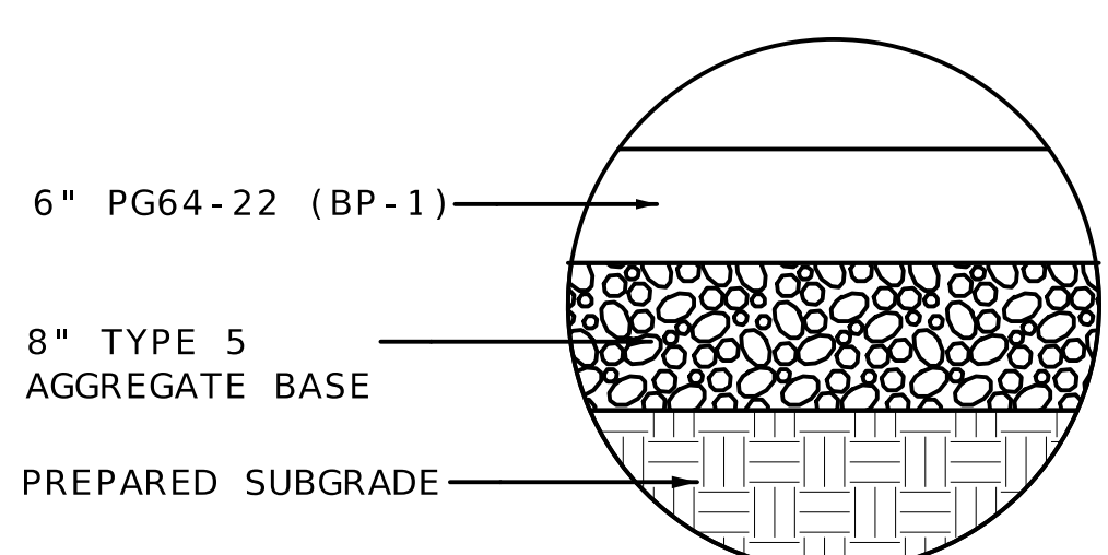
HIGH STREET FULL-DEPTH ASPHALT
