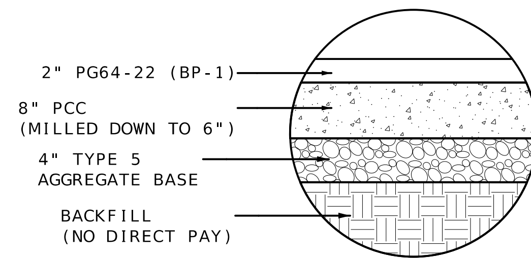
DRAINAGE INSTALLATION FULL-DEPTH CONCRETE
