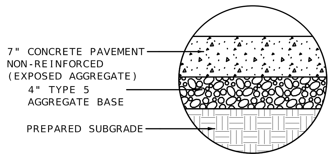
CONCRETE PARK ACCESS AND CROSSWALKS
