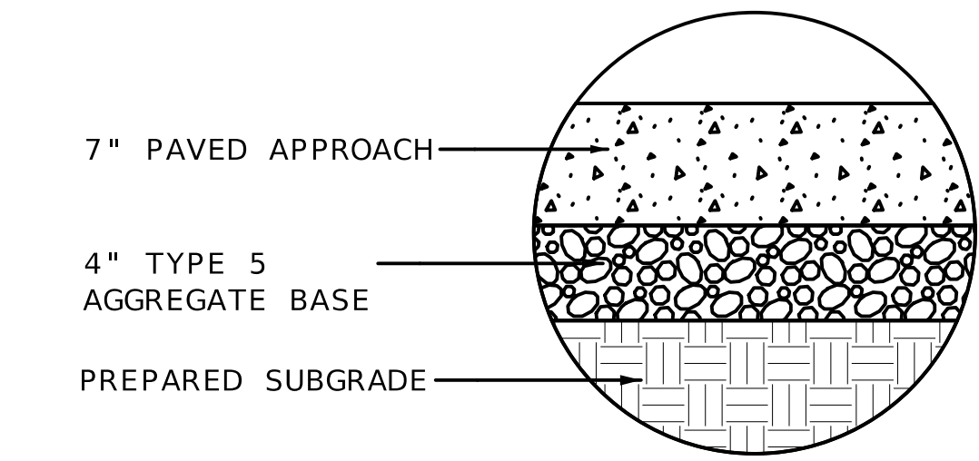
CONCRETE DRIVEWAY
