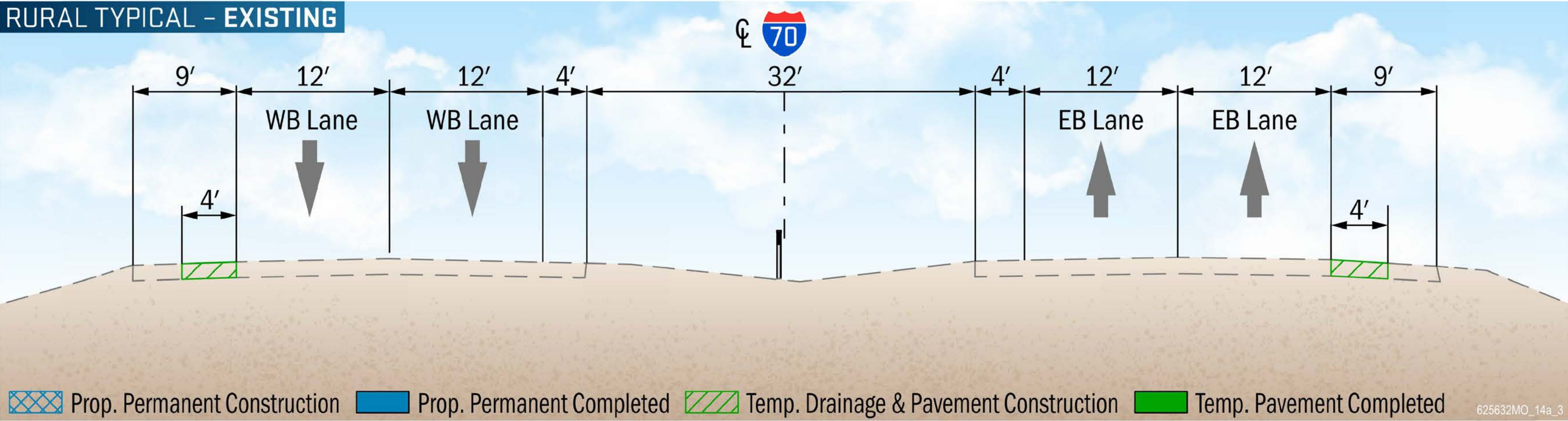
FIGURE: RURAL TYPICAL SECTIONS HIGHLIGHTS
