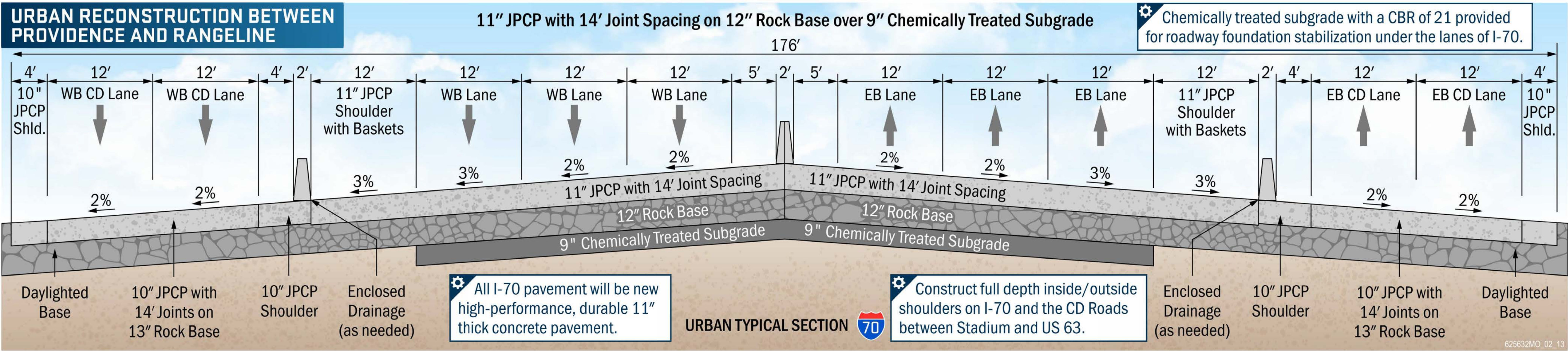
FIGURE: I-70 URBAN TYPICAL SECTION
