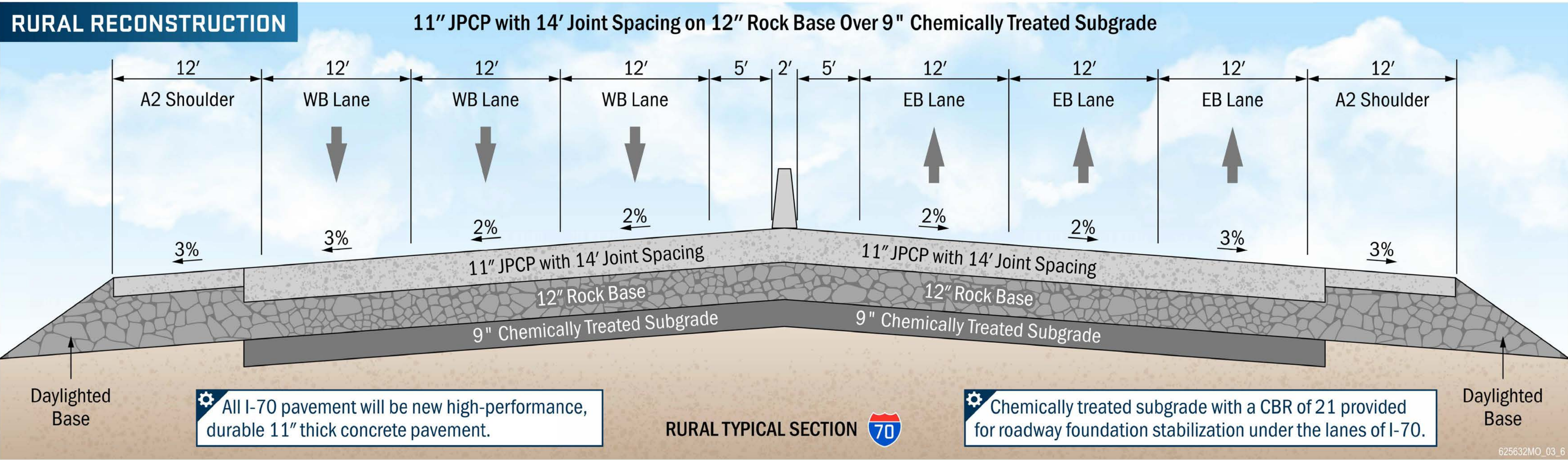
FIGURE: I-70 RURAL TYPICAL SECTION
