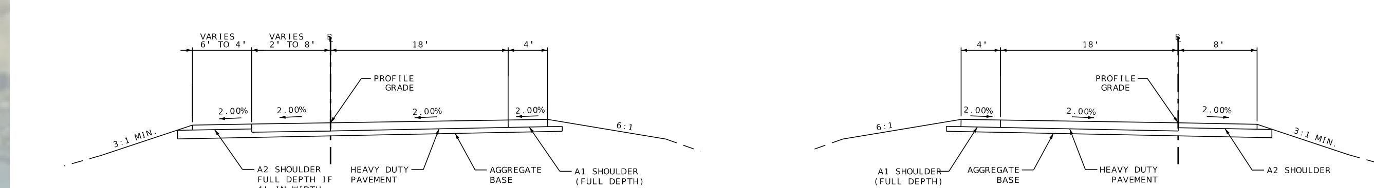
PROPOSED SECTION 149 SOUTHBOUND OFF RAMP CENTRAL STREET INTERCHANGE RAMP 2 - STA. 6+60.00 TO STA. 7+75.00
