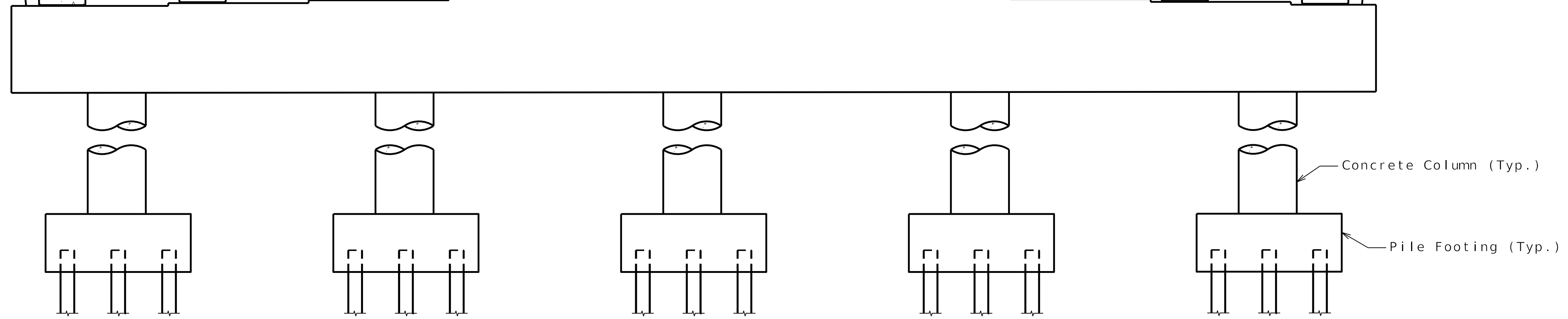
PROPOSED TYPICAL SECTION AT INTERMEDIATE BENT
