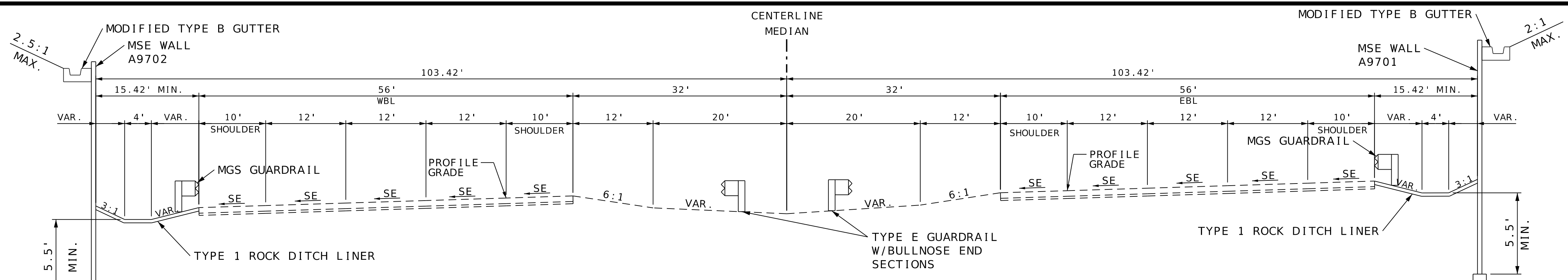
SECTION ON SUPERELEVATED CURVE TYPICAL SECTION RTE. 1435 STA. 944+39.92 TO STA. 945+38.92
