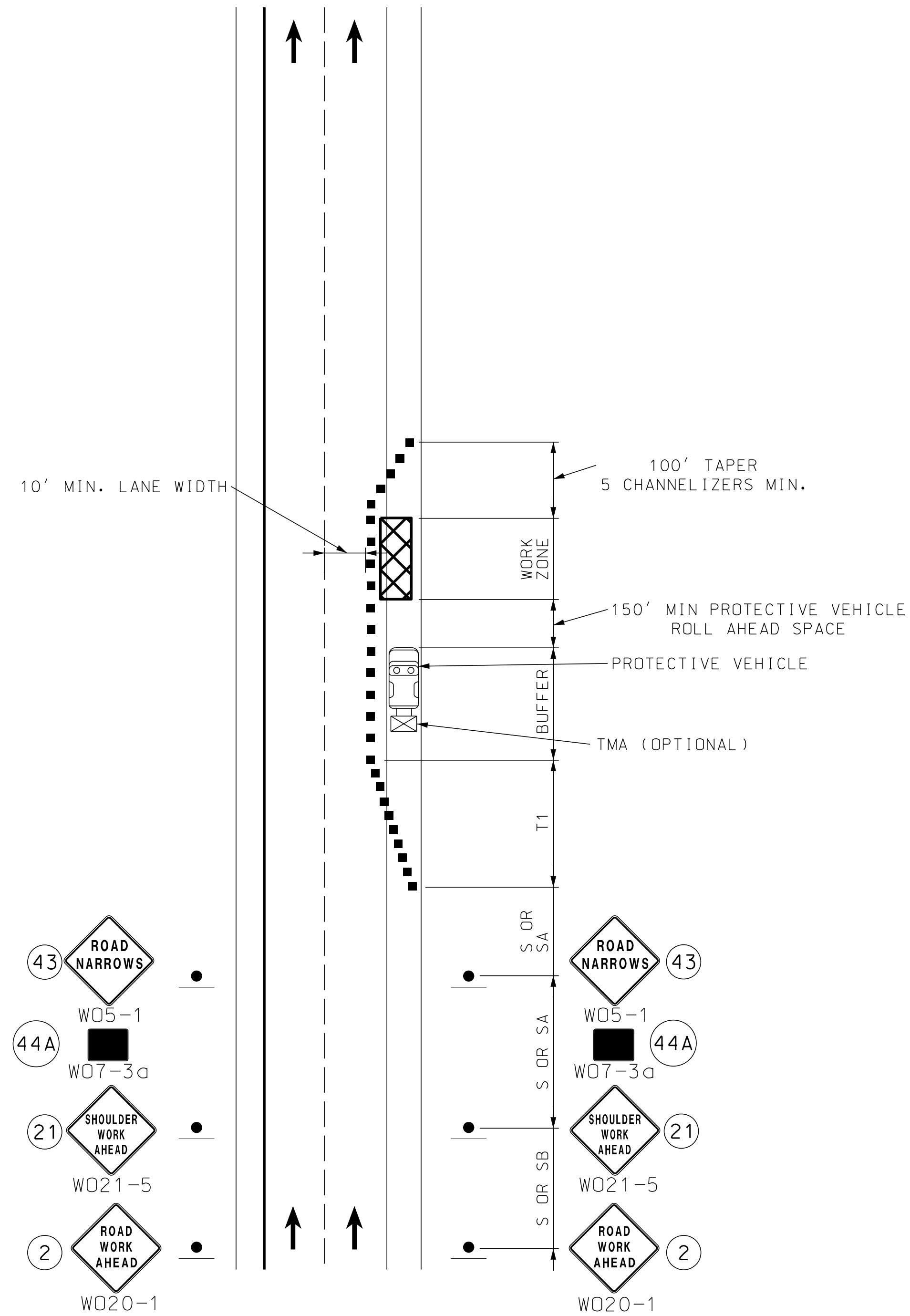
I-435 SHOULDER WORK WITH MINOR ENCROACHMENT ON DIVIDED AND UNDIVIDED HIGHWAYS
