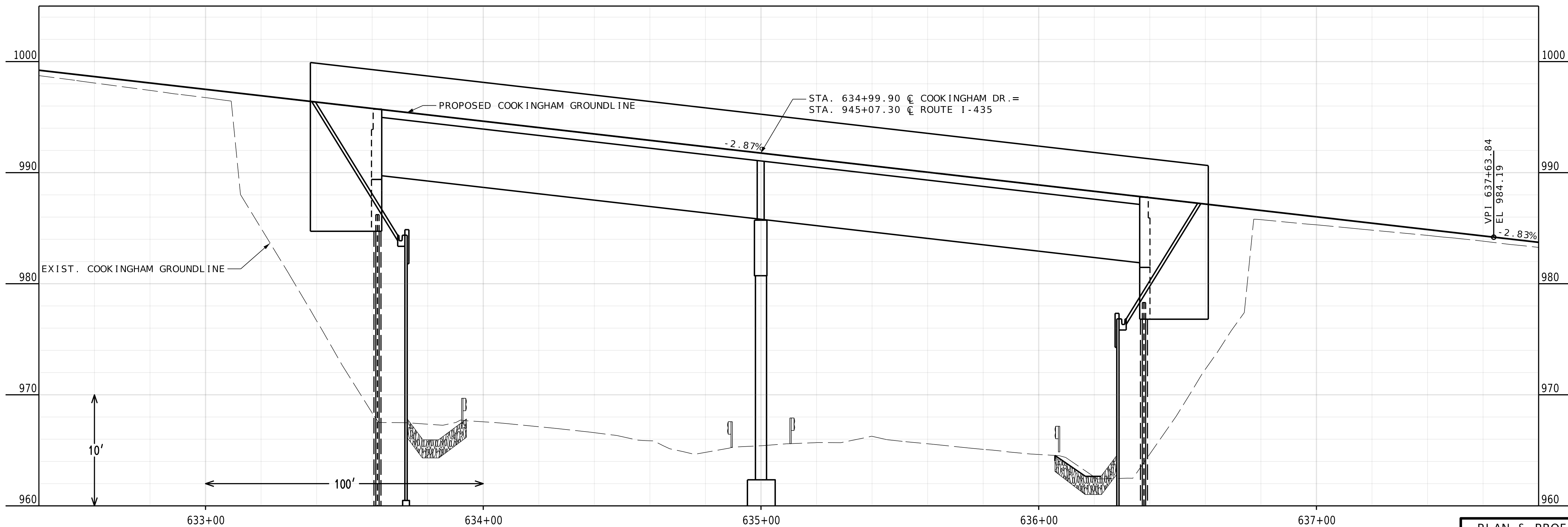
PLAN & PROFILE SHEET 7 OF 8
