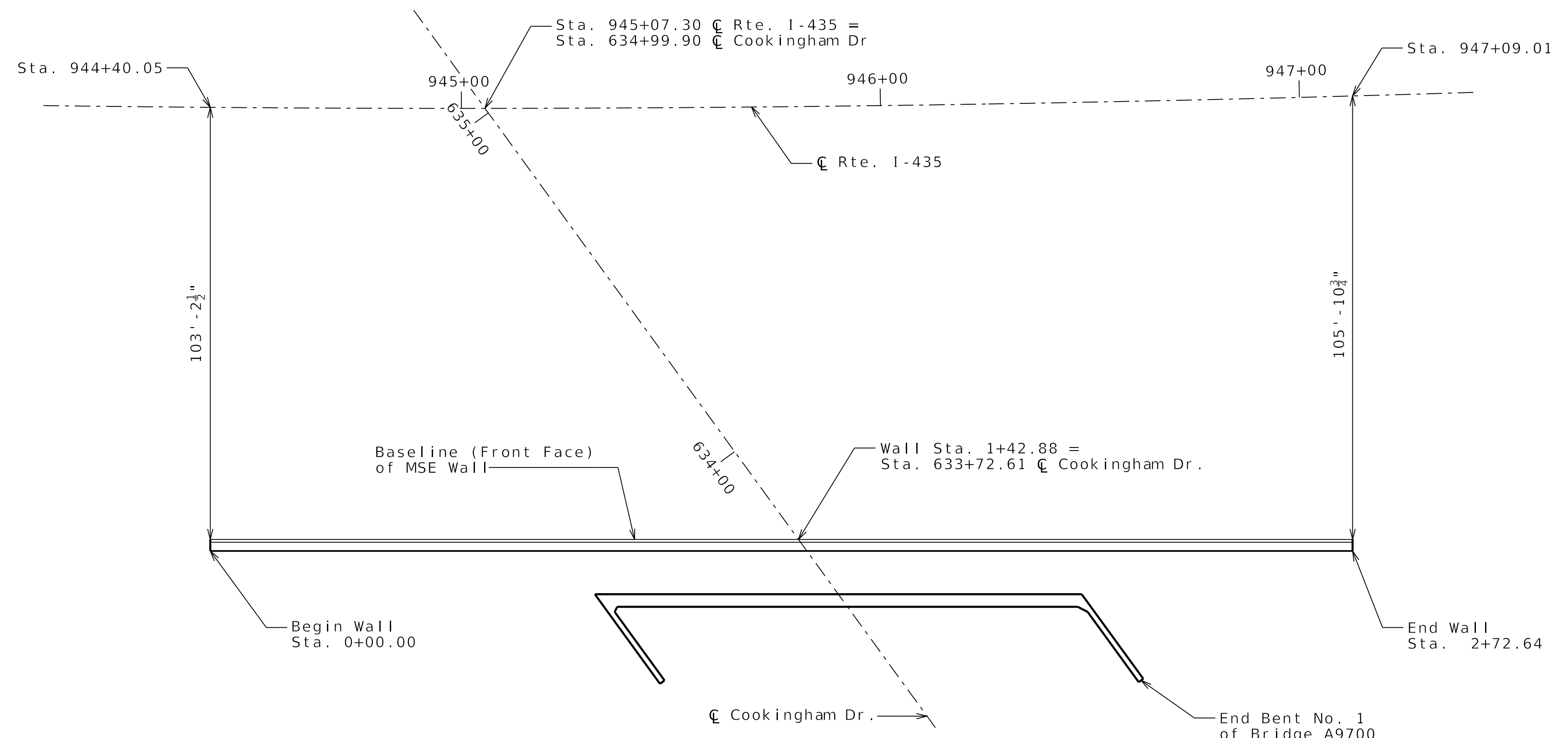
PLAN Concrete Leveling pad and Coping not shown for clarity.
