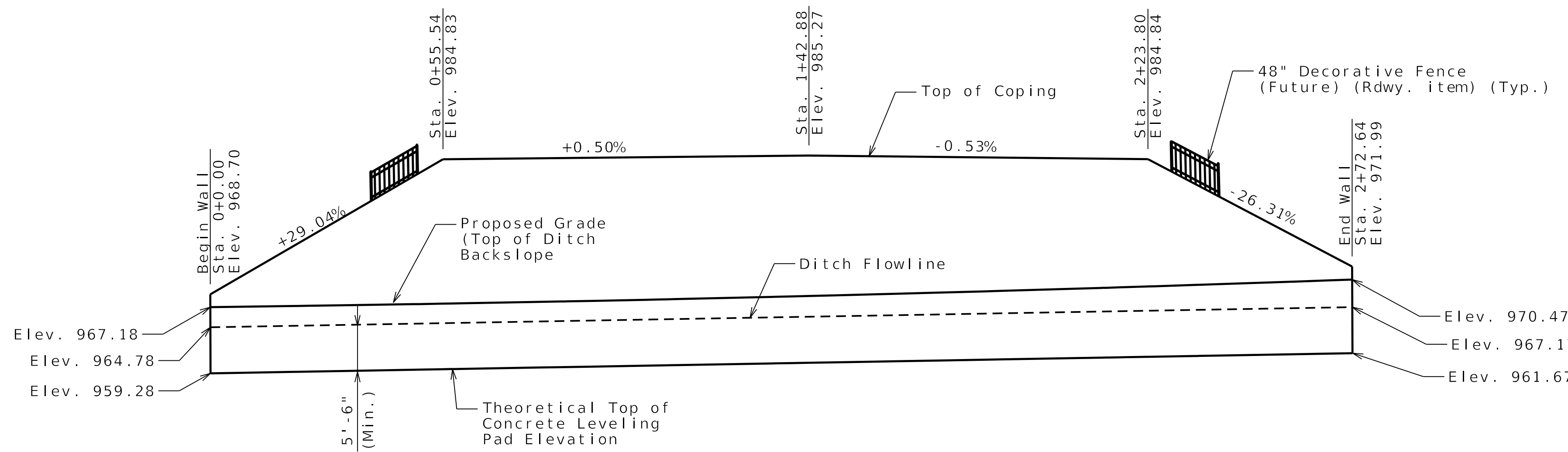
DEVELOPED ELEVATION Concrete Leveling pad and Coping not shown for clarity.
