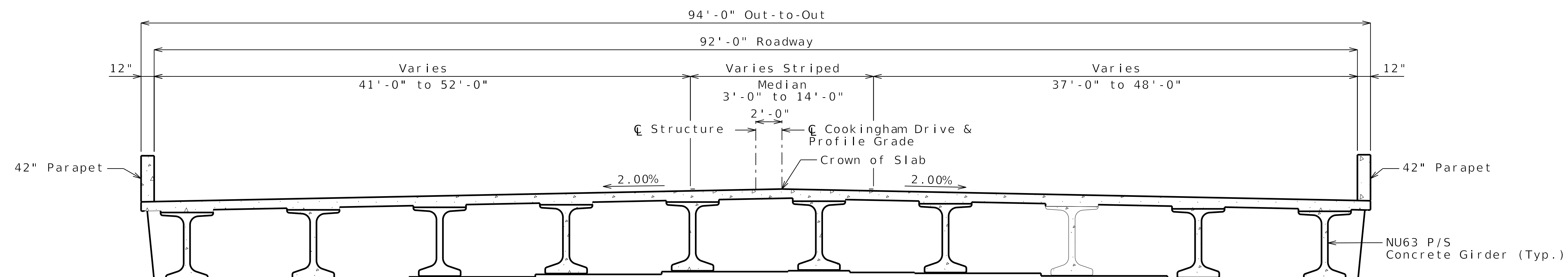
FUTURE TYPICAL SECTION
