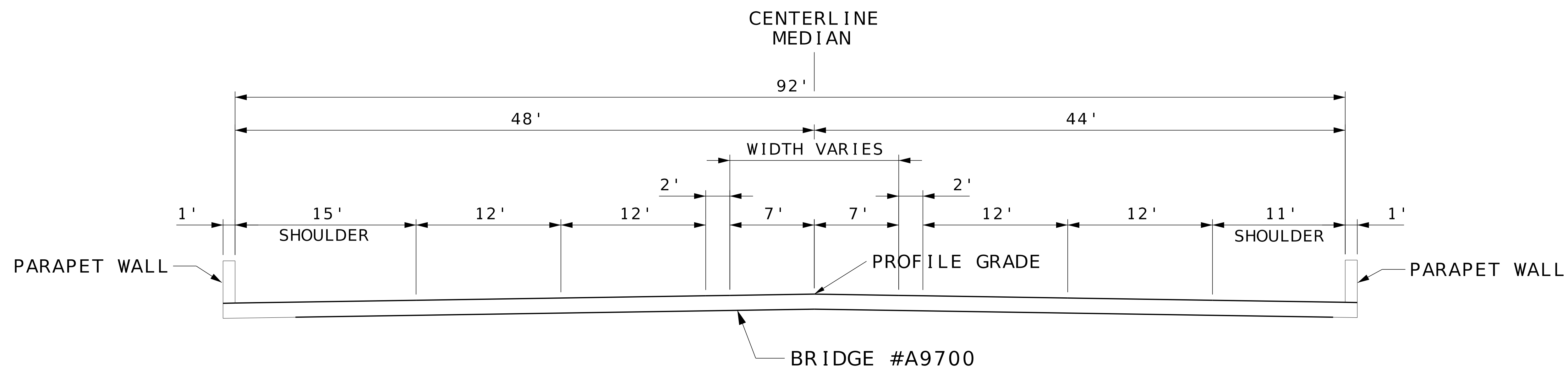
SECTION ON TANGENT TYPICAL SECTION BRIDGE STA. 633+53.35 TO STA. 636+46.45
