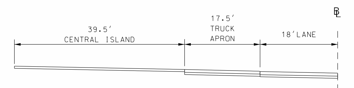
PROPOSED ROUNDABOUT TYPICAL SECTION
