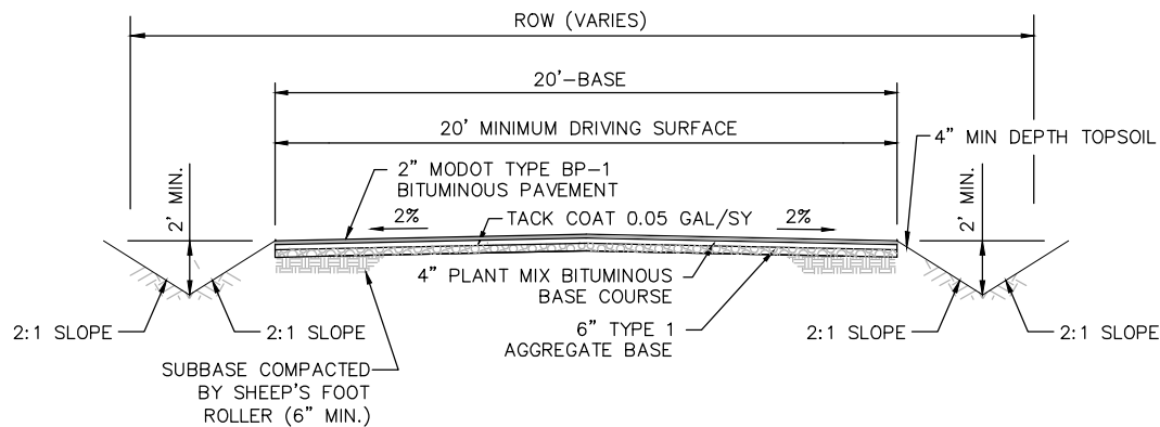
TYPICAL ASPHALT PAVEMENT SECTION
