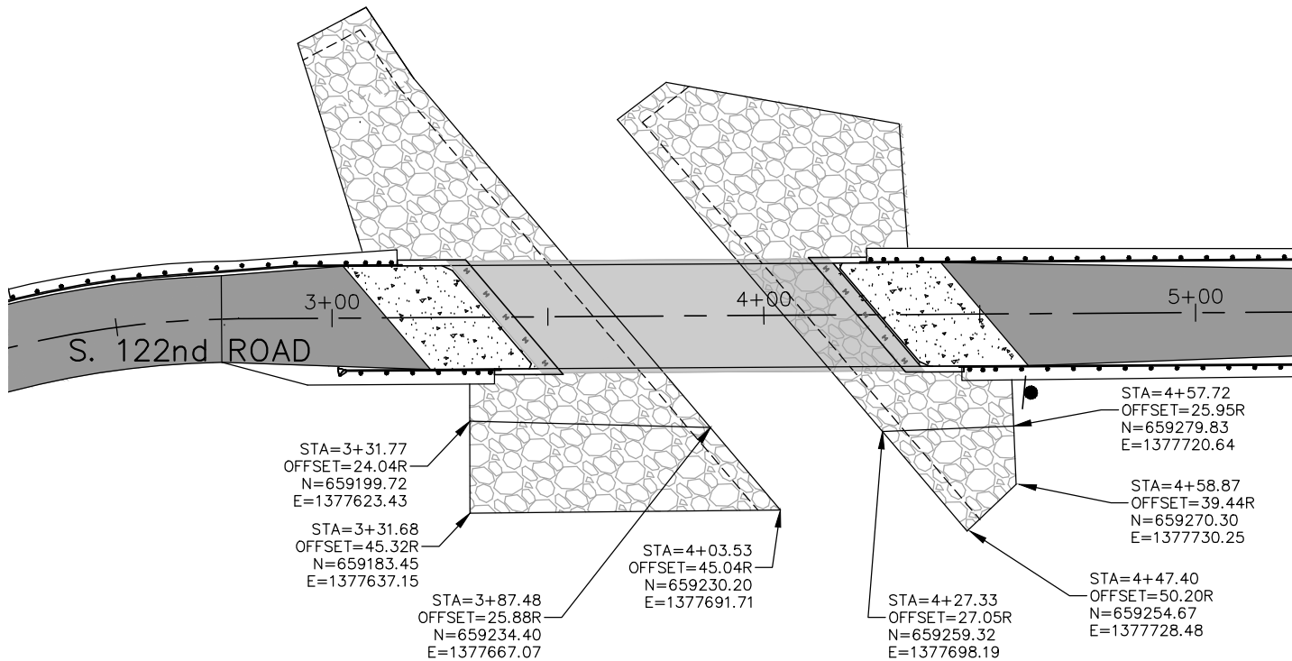
MODOT TYPE 2 ROCK BLANKET LAYOUT PLAN
