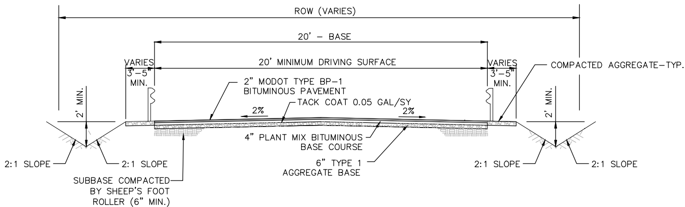
TYPICAL ASPHALT PAVEMENT SECTION W/ GUARDRAIL
