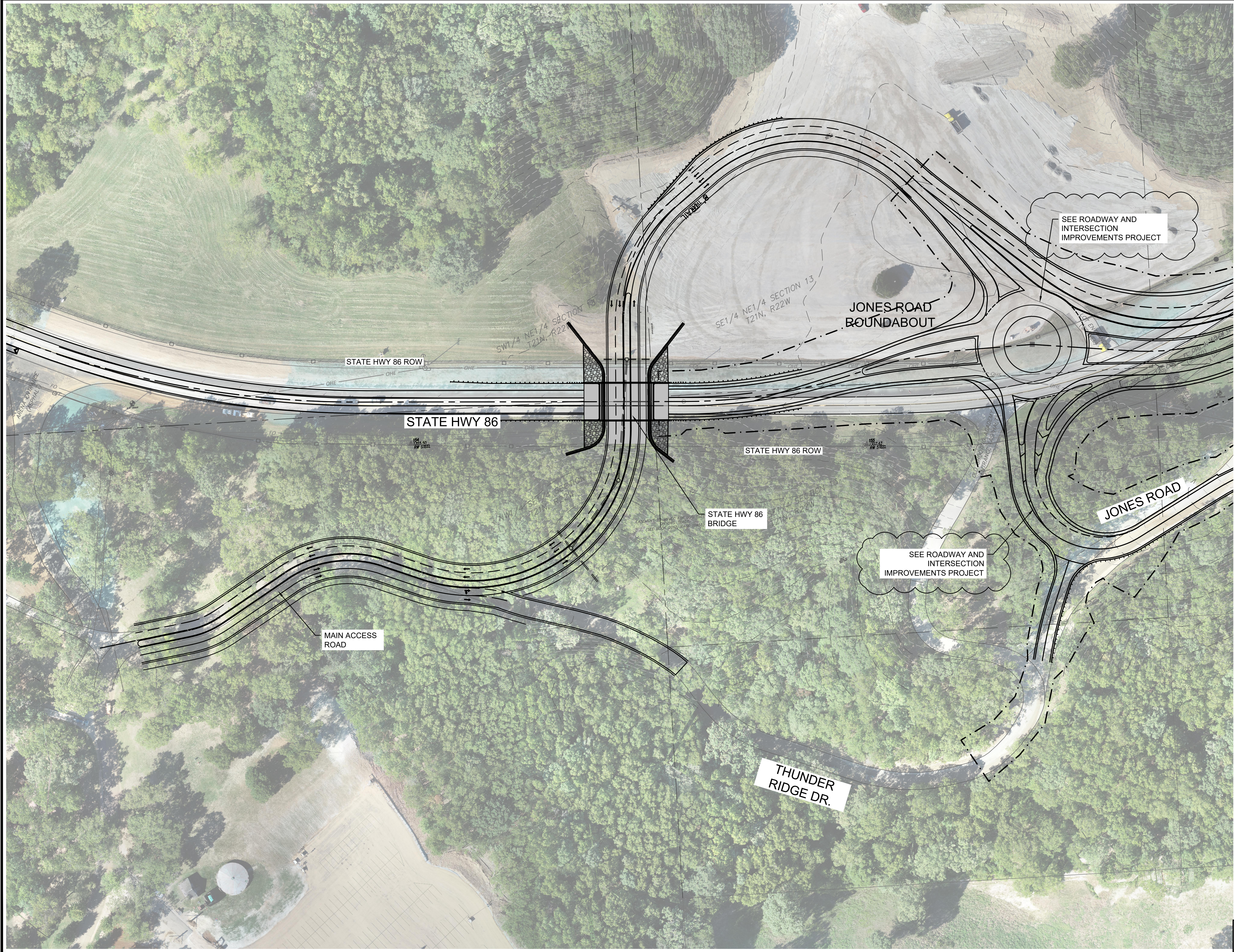
HWY 86 BRIDGE AND MAIN ACCESS ROAD SHEET 1 OF 1 OVERALL PLAN
