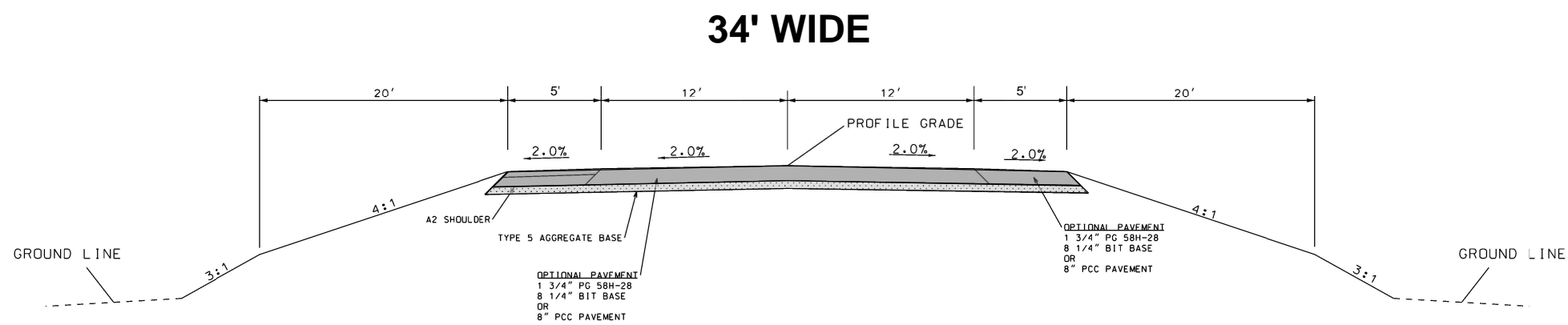
PROPOSED ROUTE 6 ROADWAY
