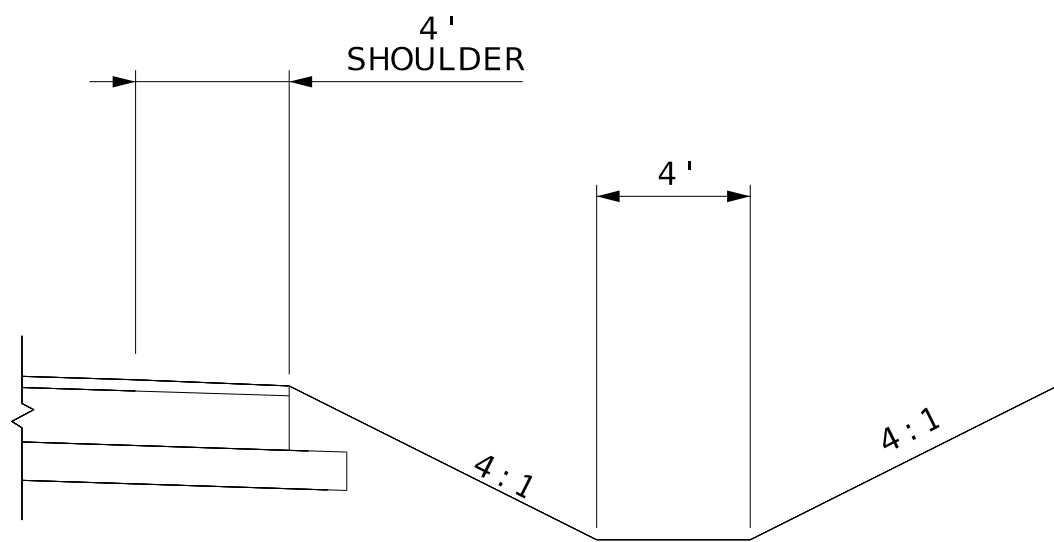
SHOULDER DETAIL RT
