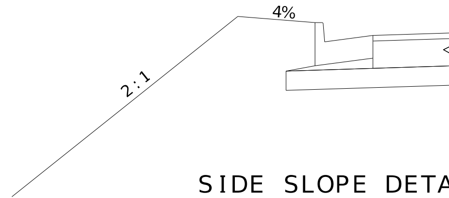
SIDE SLOPE DETAIL LT
