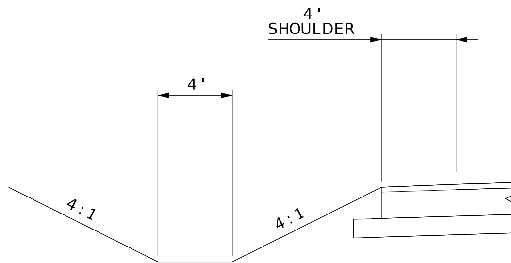
SHOULDER DETAIL LT
