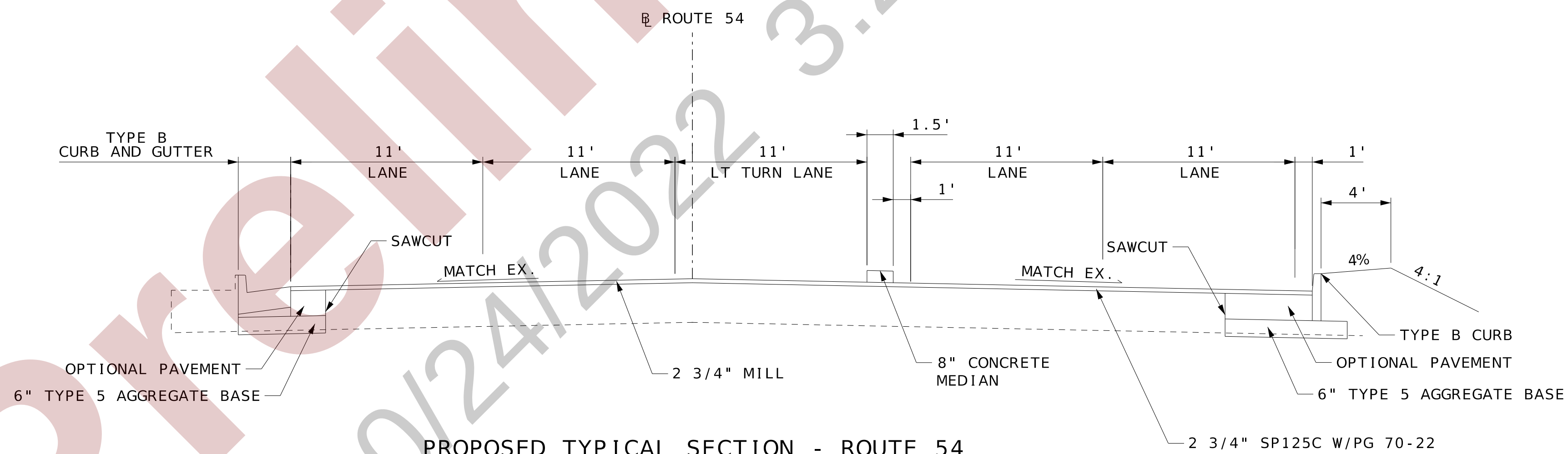
PROPOSED TYPICAL SECTION - ROUTE 54
