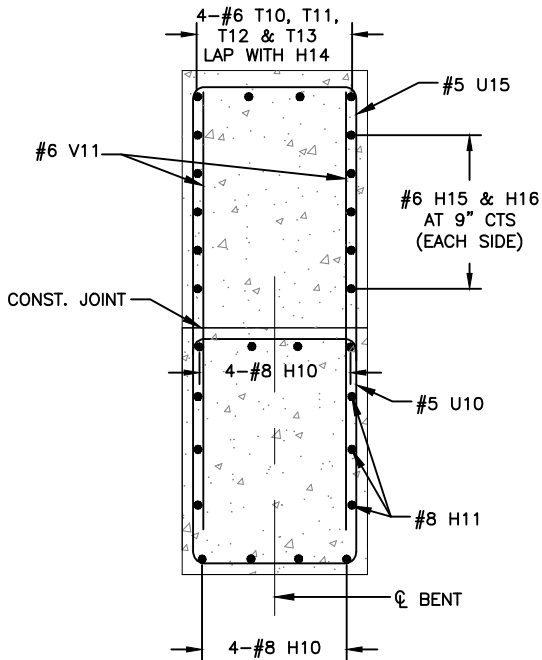
SECTION THROUGH WING
