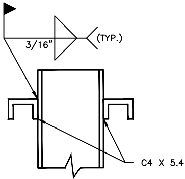
FRONT ELEVATION
