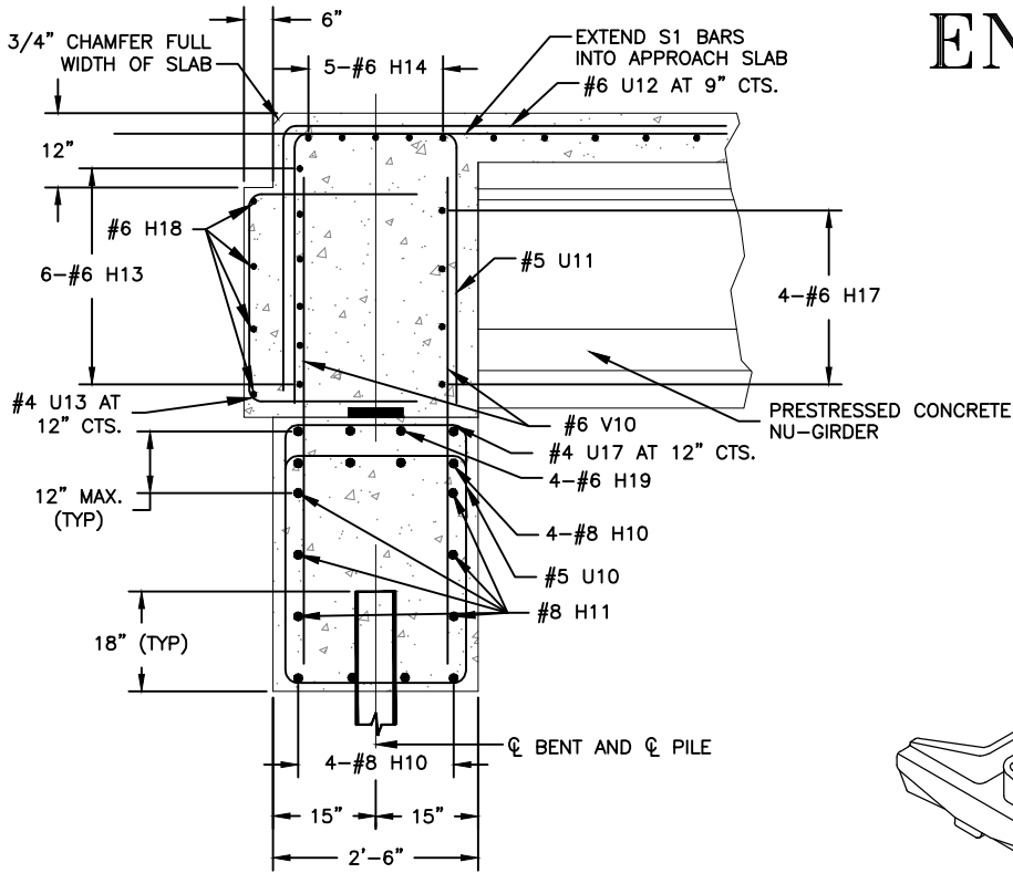
SECTION BETWEEN GIRDERS
