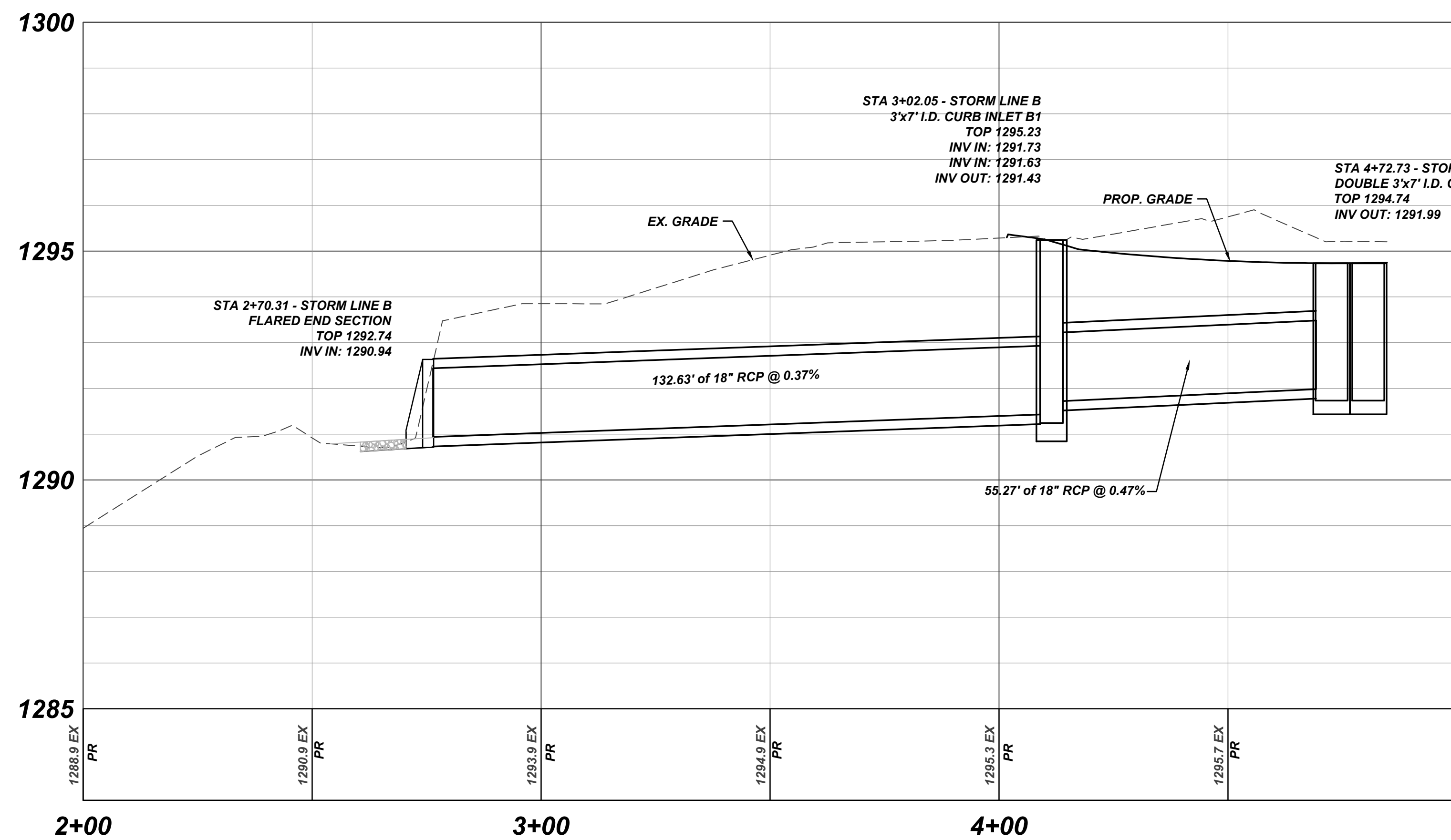
STORM LINE B PROFILE SCALE: 1"=20'
