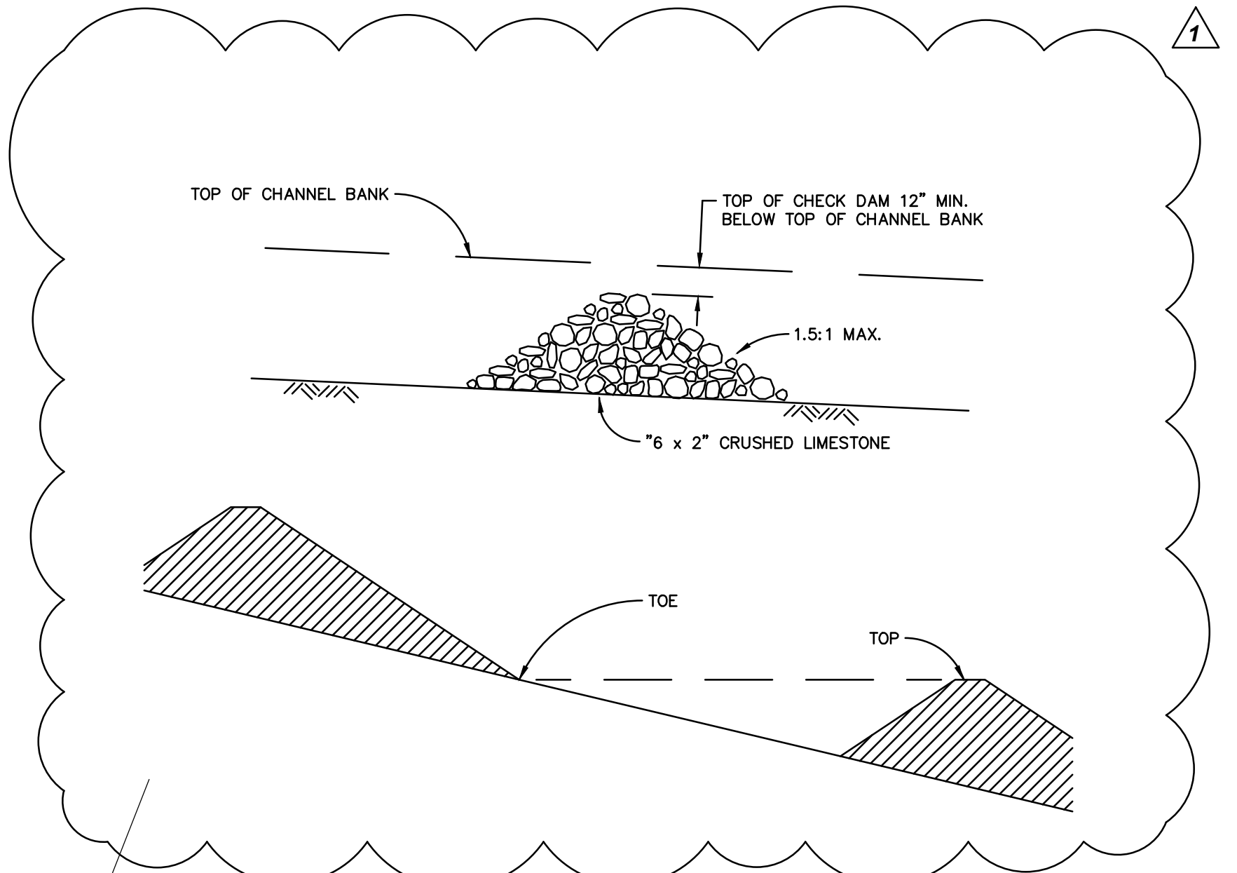
ROCK DITCH CHECK NOT TO SCALE
