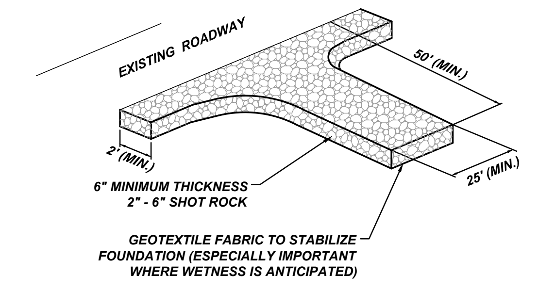
TEMPORARY CONSTRUCTION ENTRANCE NOT TO SCALE
