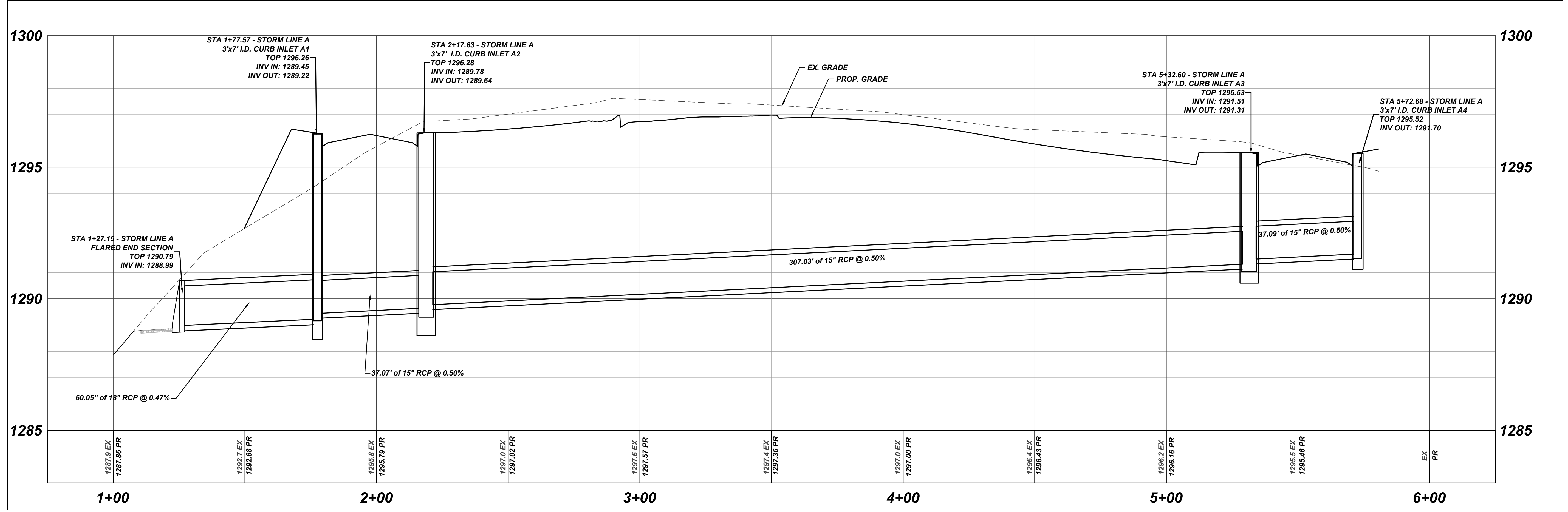
STORM LINE A PROFILE SCALE: 1"=20'
