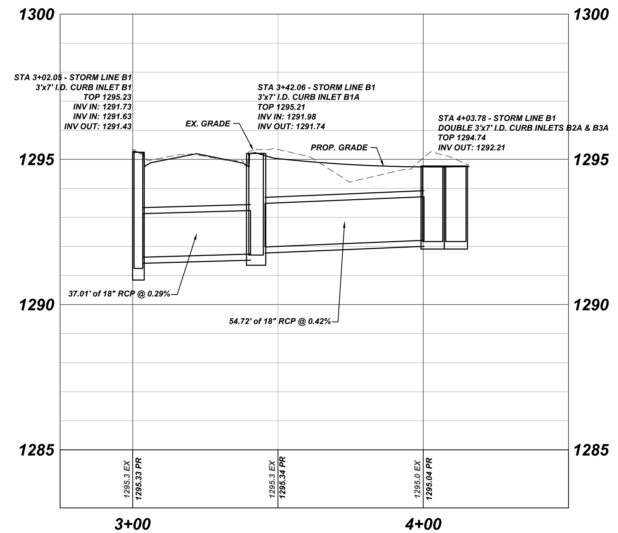
STORM LINE B1 PROFILE SCALE: 1"=20'
