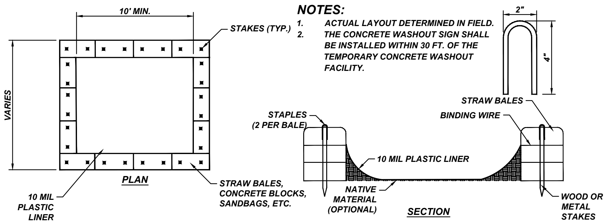
TEMPORARY CONCRETE WASHOUT DETAIL NOT TO SCALE
