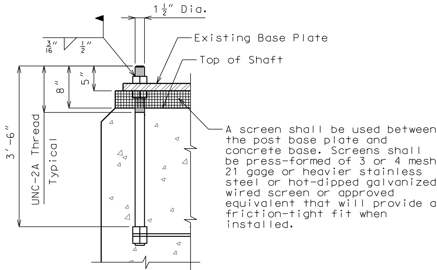
ANCHOR BOLT DETAIL
