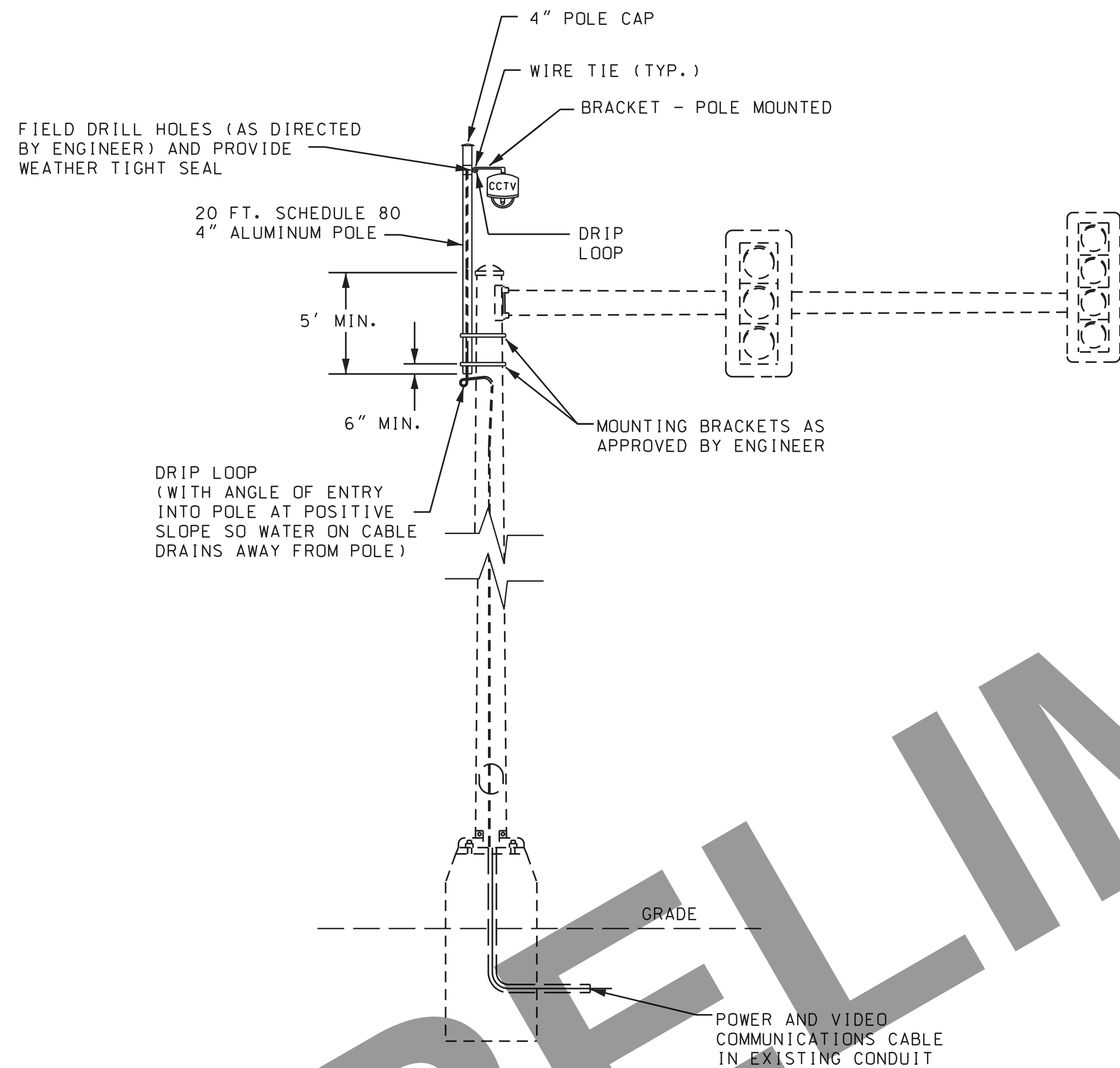
CCTV MOUNTING ON SIGNAL POLE WITH NEW EXTENSION
