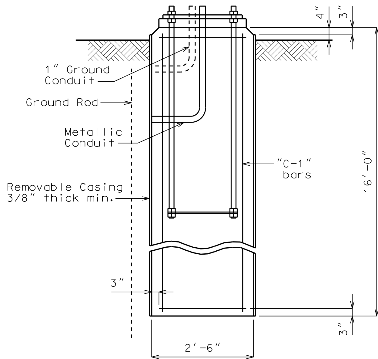
TYPICAL CAMERA POLE
