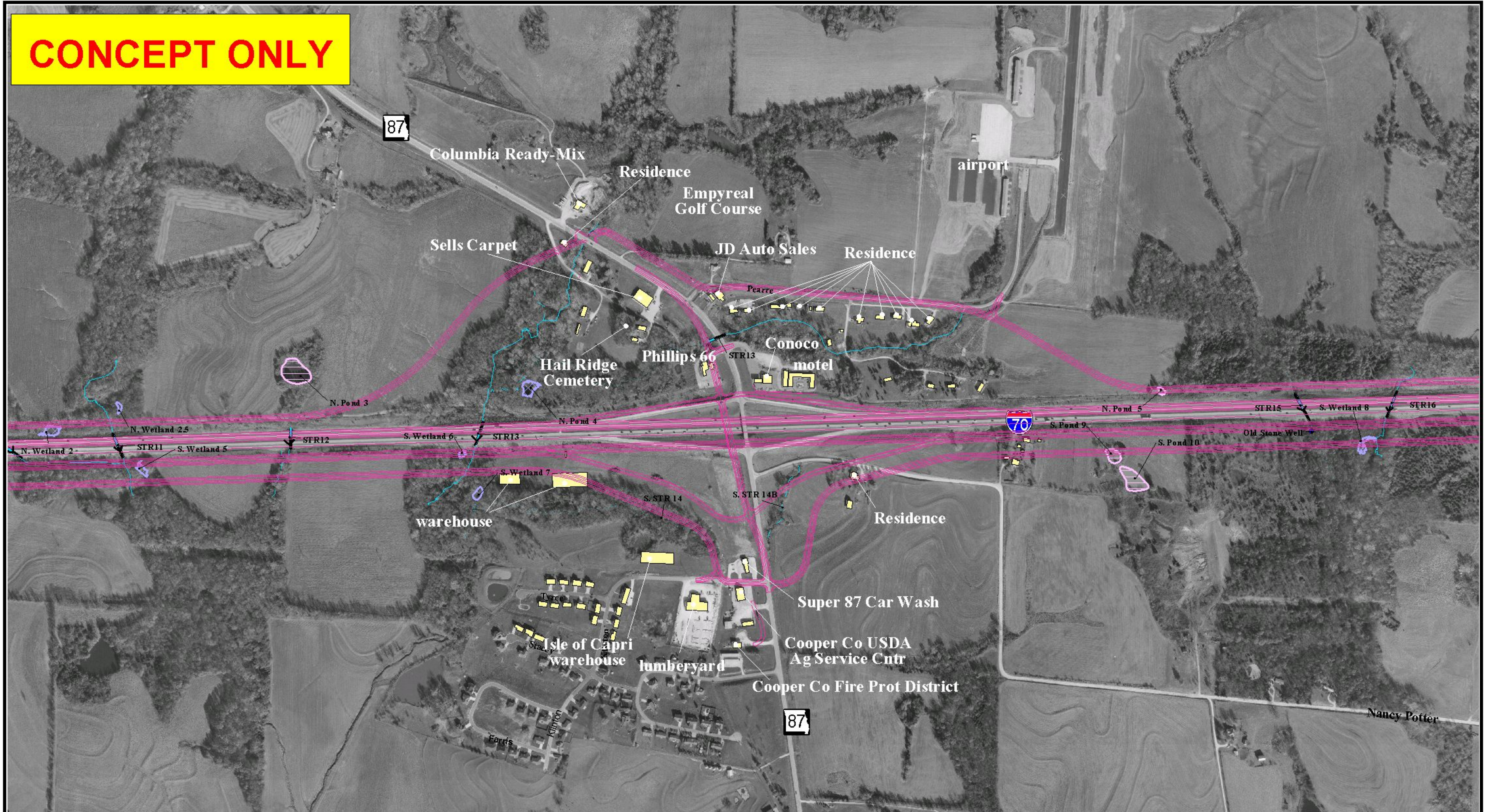
Figure 9 Interchange Concept Option 3 Route 87
