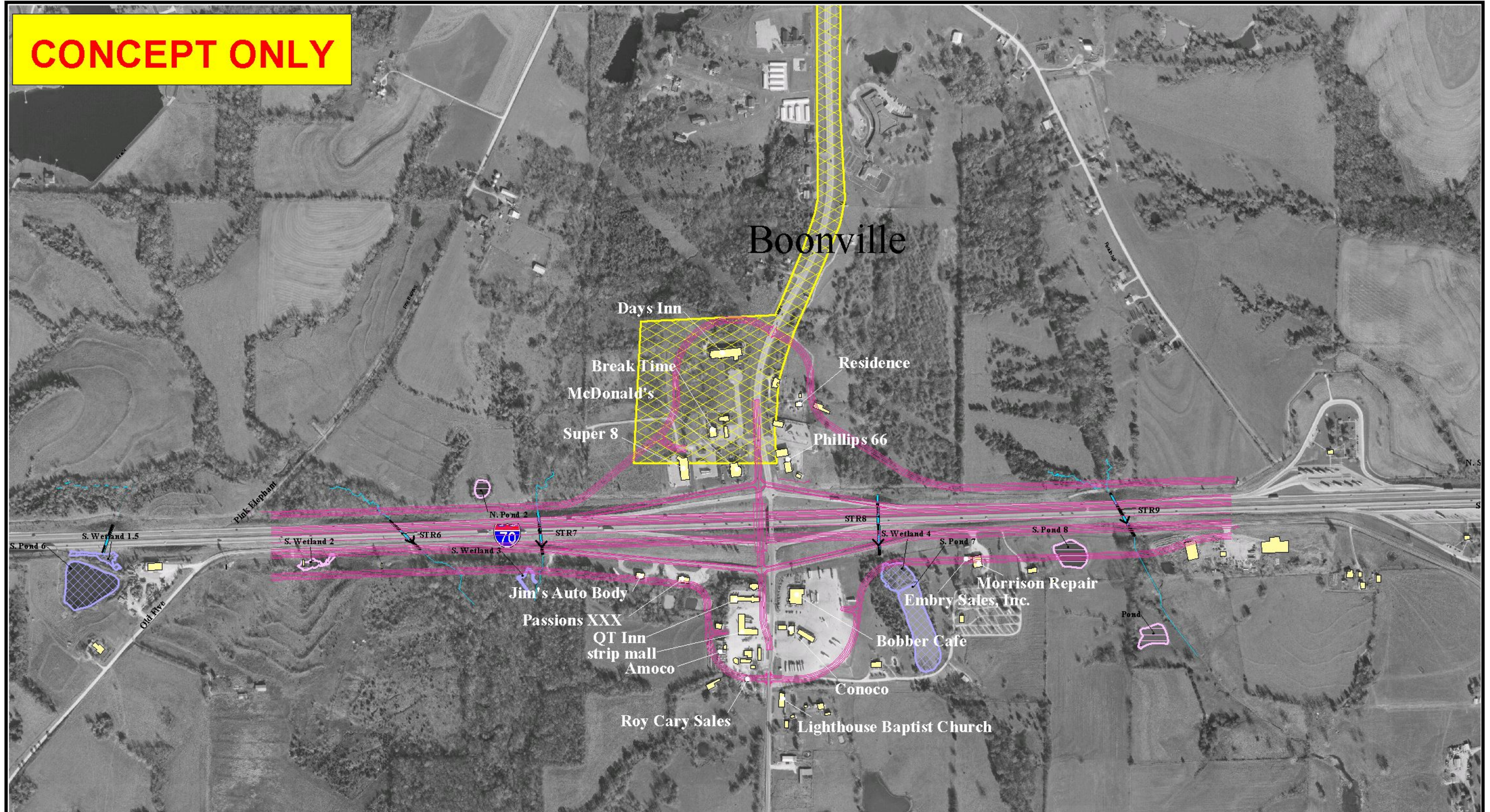
Figure 6 Interchange Concept Option 3 Route B
