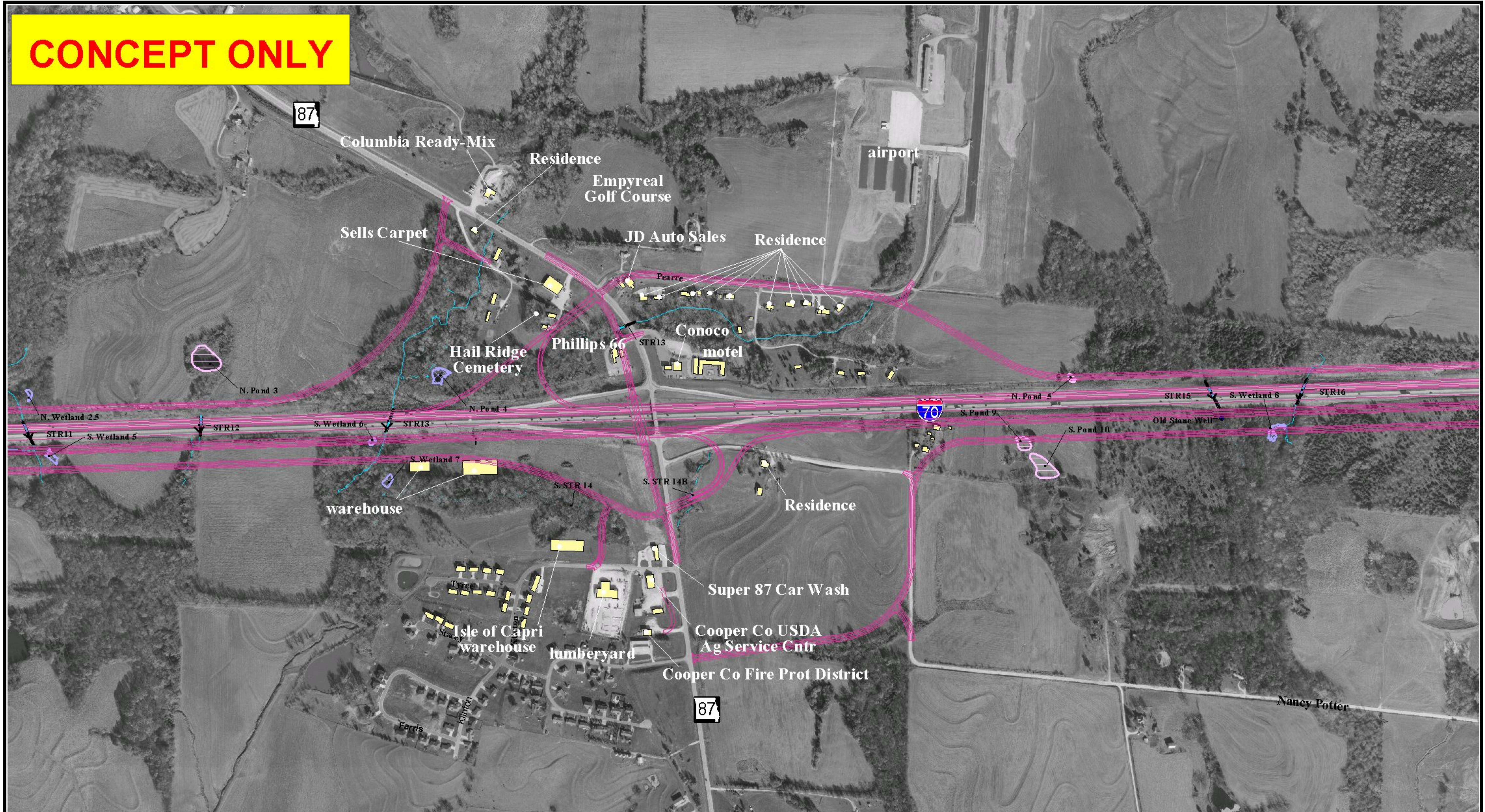
Figure 8 Interchange Concept Option 2 Route 87
