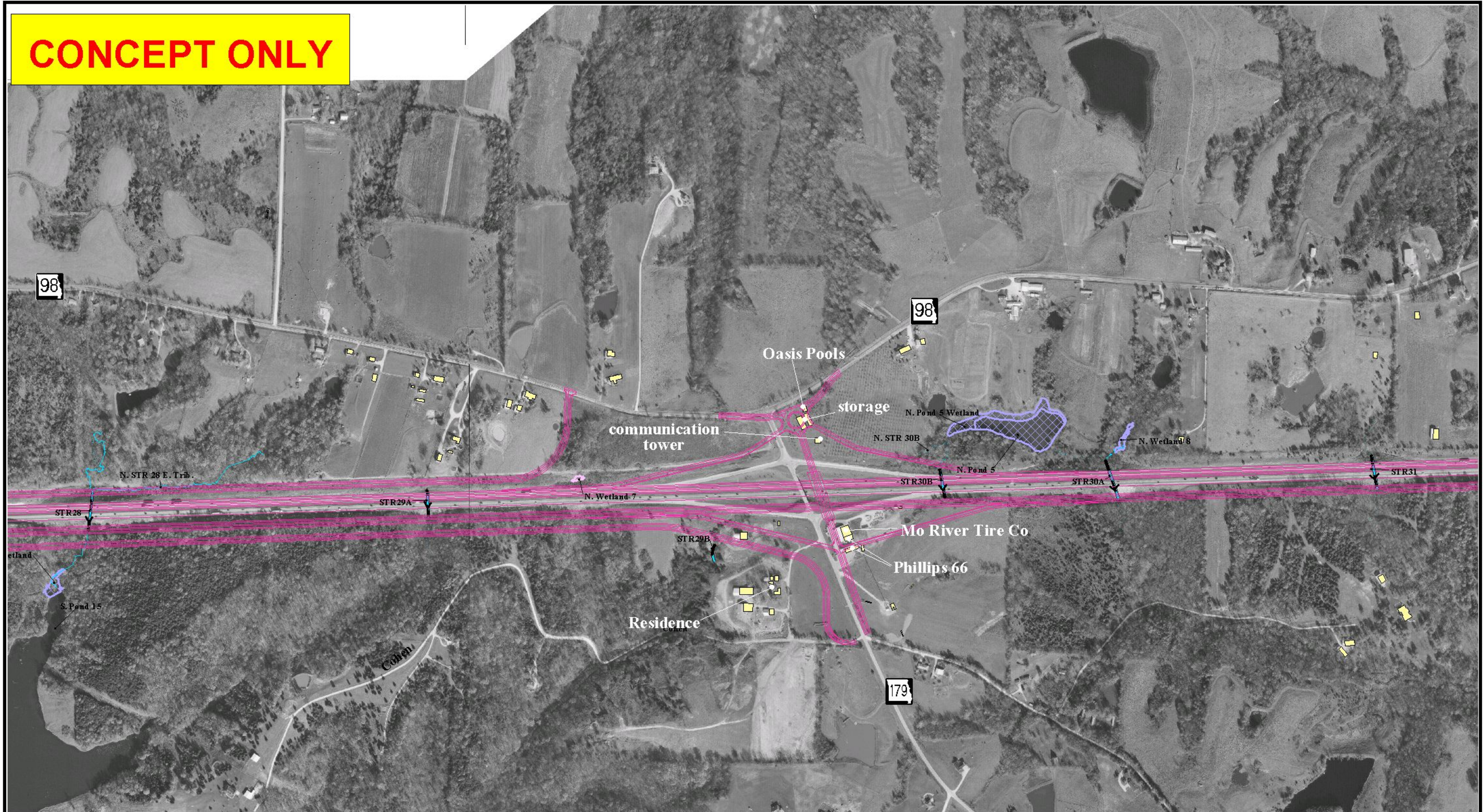
Figure 11 Interchange Concept Route 179
