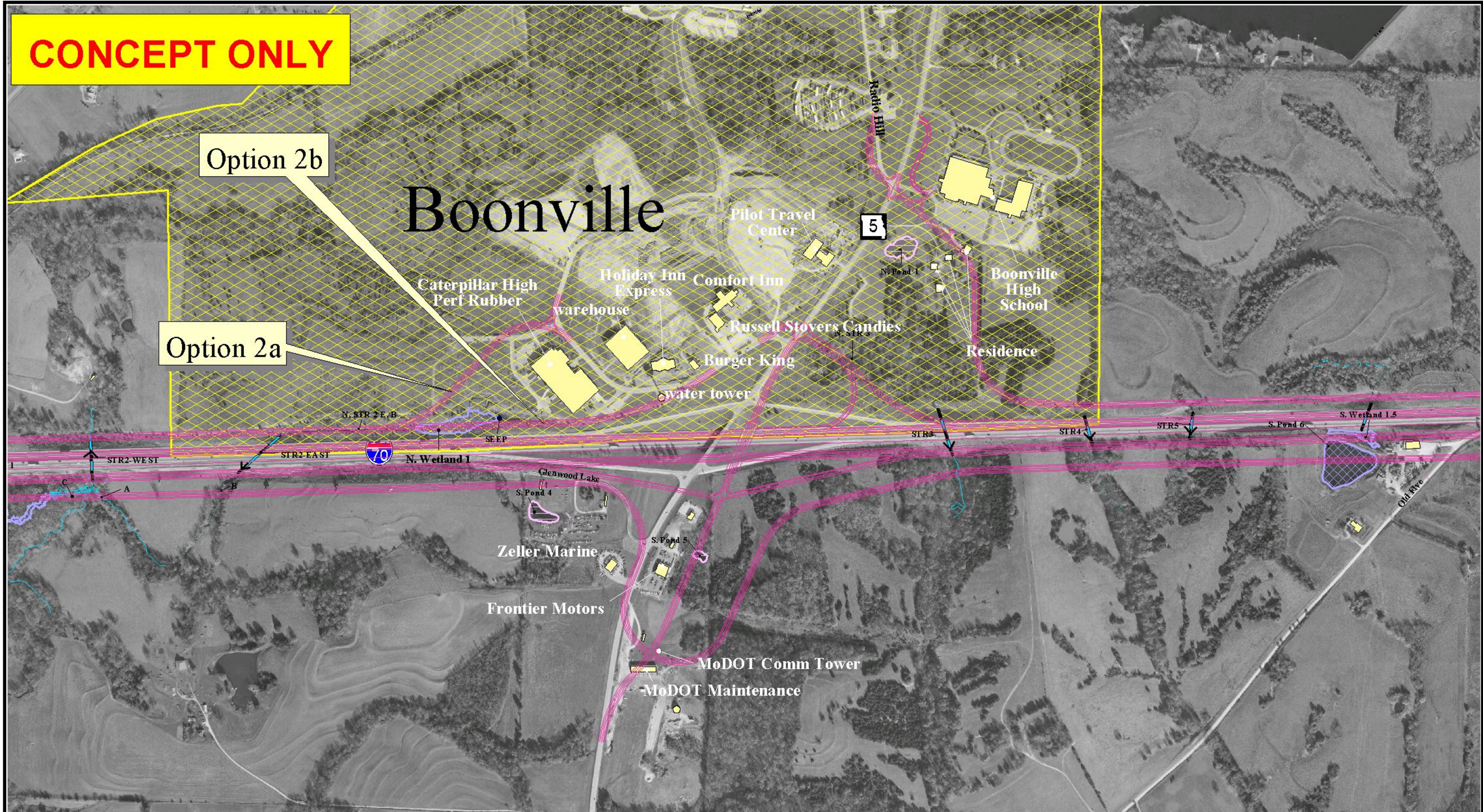
Figure 2 Interchange Concept Option 2 Route 5
