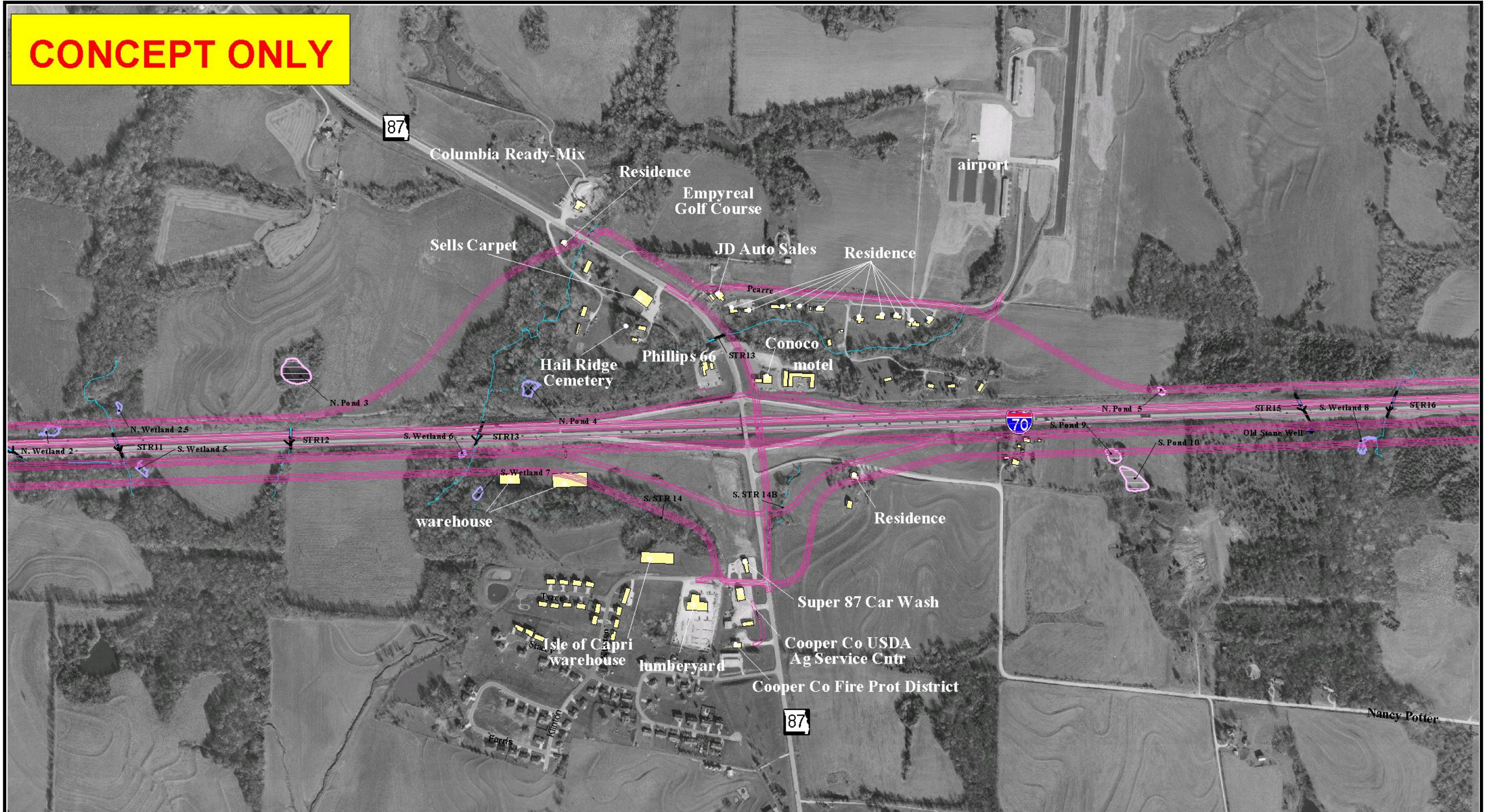
Figure 10 Interchange Concept Option 4 Route 87
