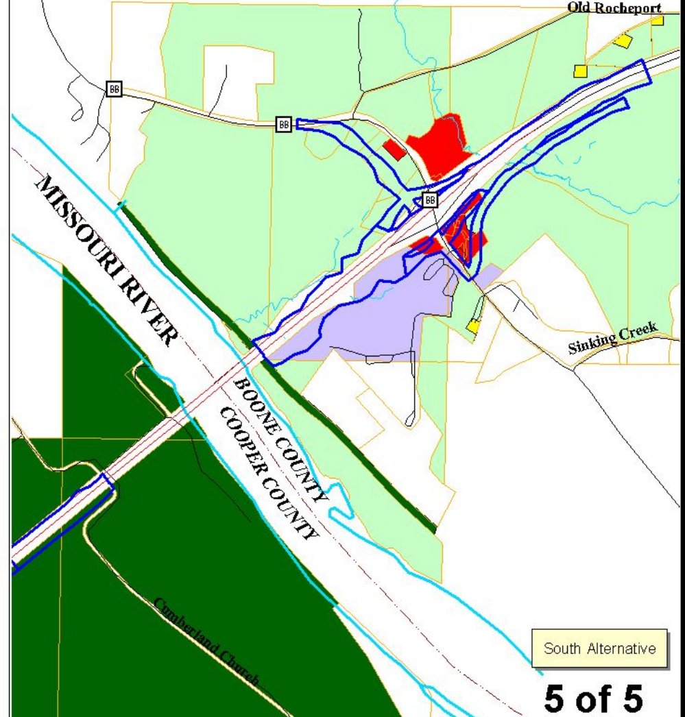
Figure III-3 Land Use Cooper & Boone Counties, Missouri
