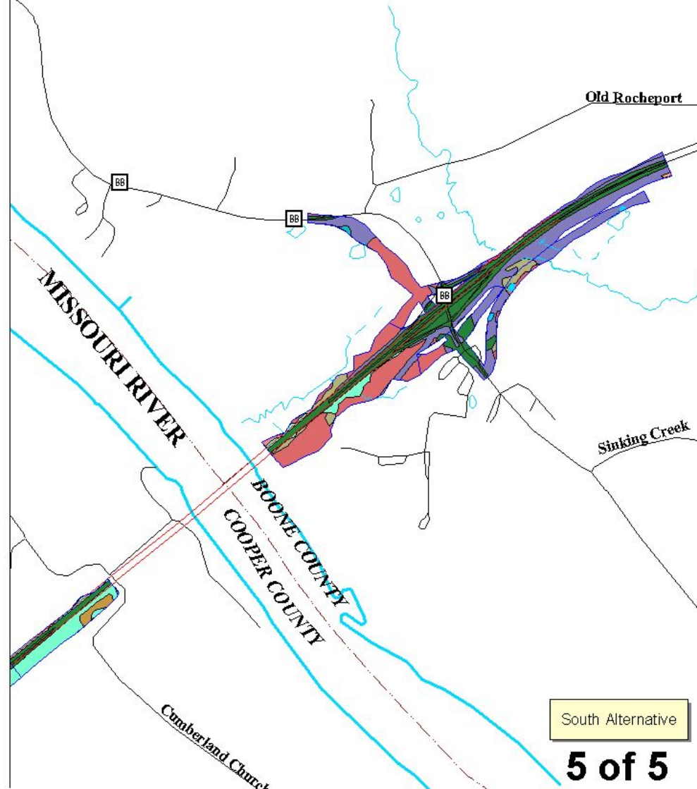
Figure III-4 Land Cover Cooper & Boone Counties, Missouri
