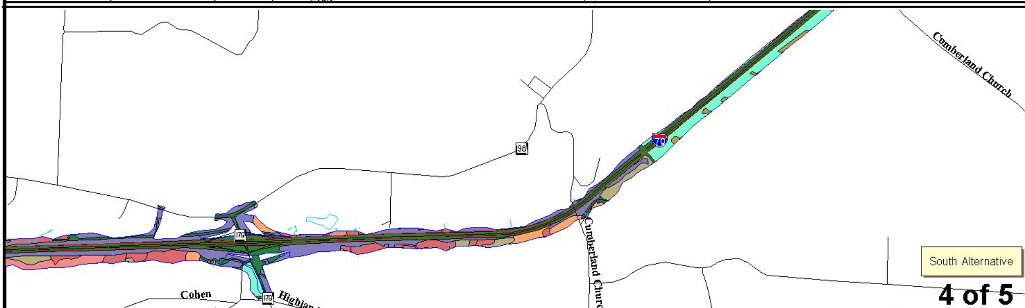
Figure III-4 Land Cover Cooper & Boone Counties, Missouri
