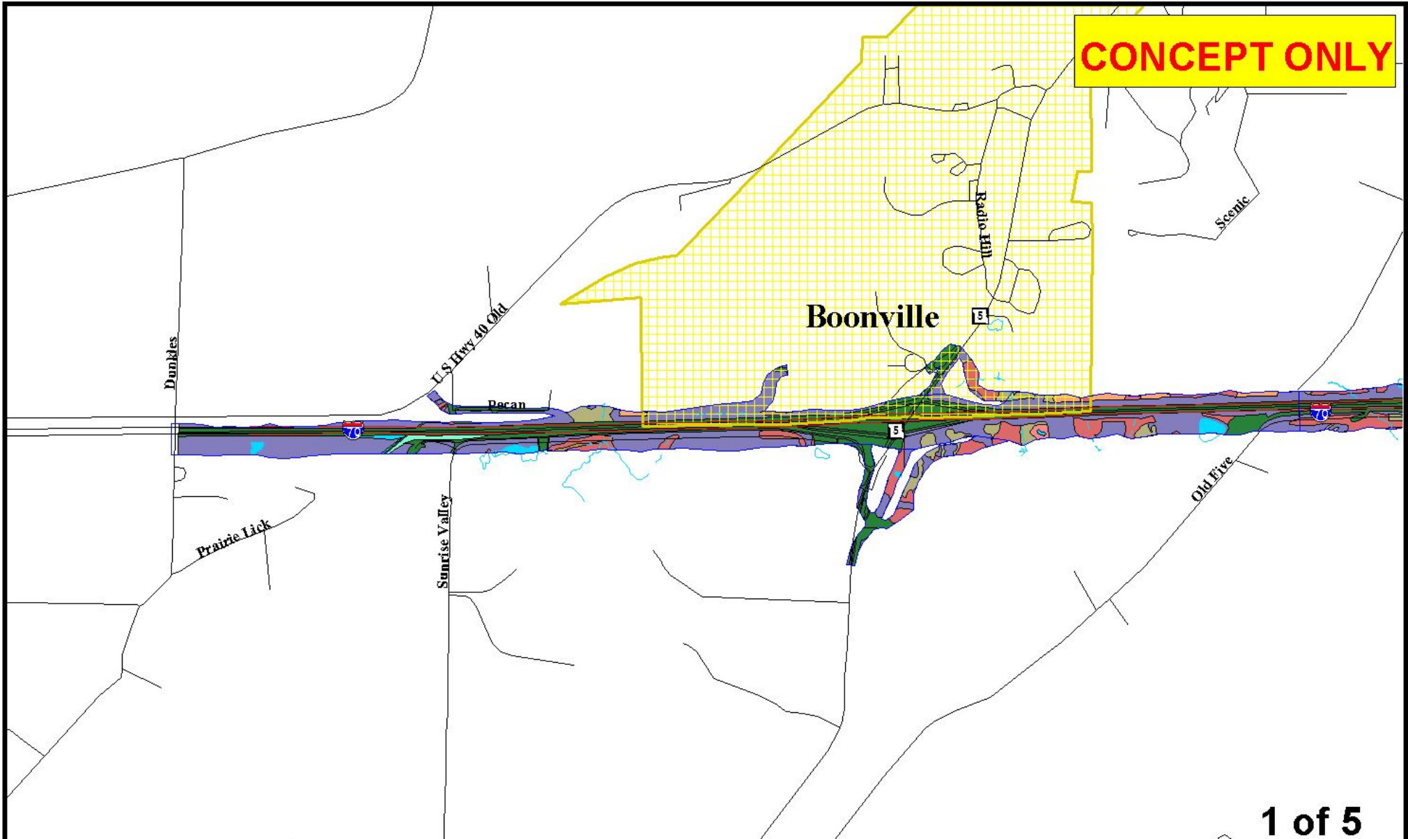
Figure III-4 Land Cover Cooper & Boone Counties, Missouri
