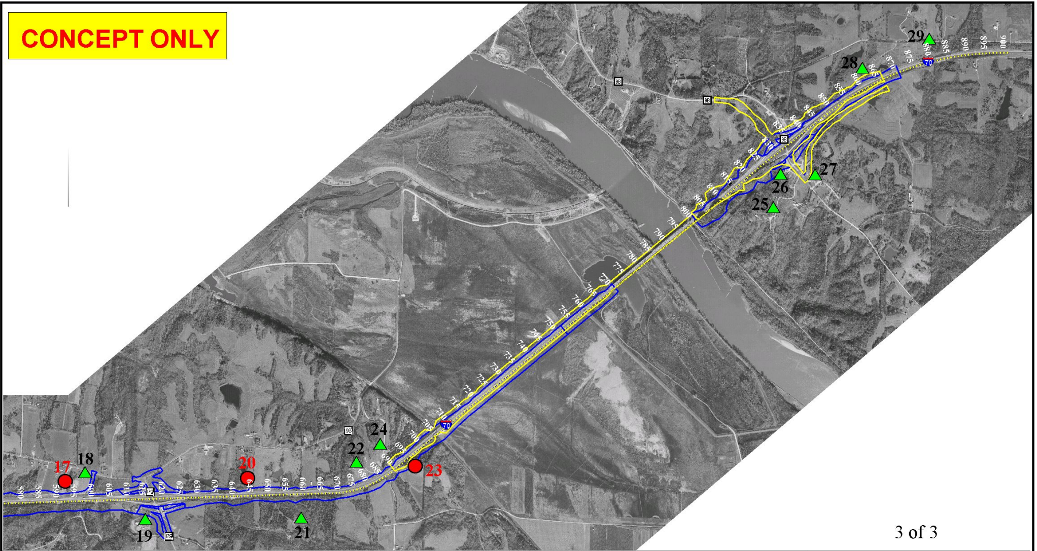
Figure III-5 Noise Analysis Receptors Cooper & Boone Counties, Missouri
