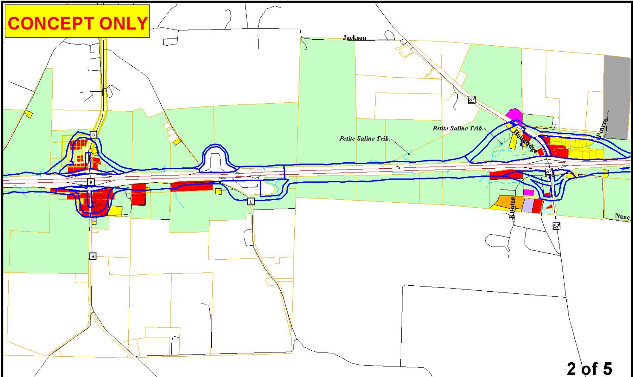
Figure III-3 Land Use Cooper & Boone Counties, Missouri
