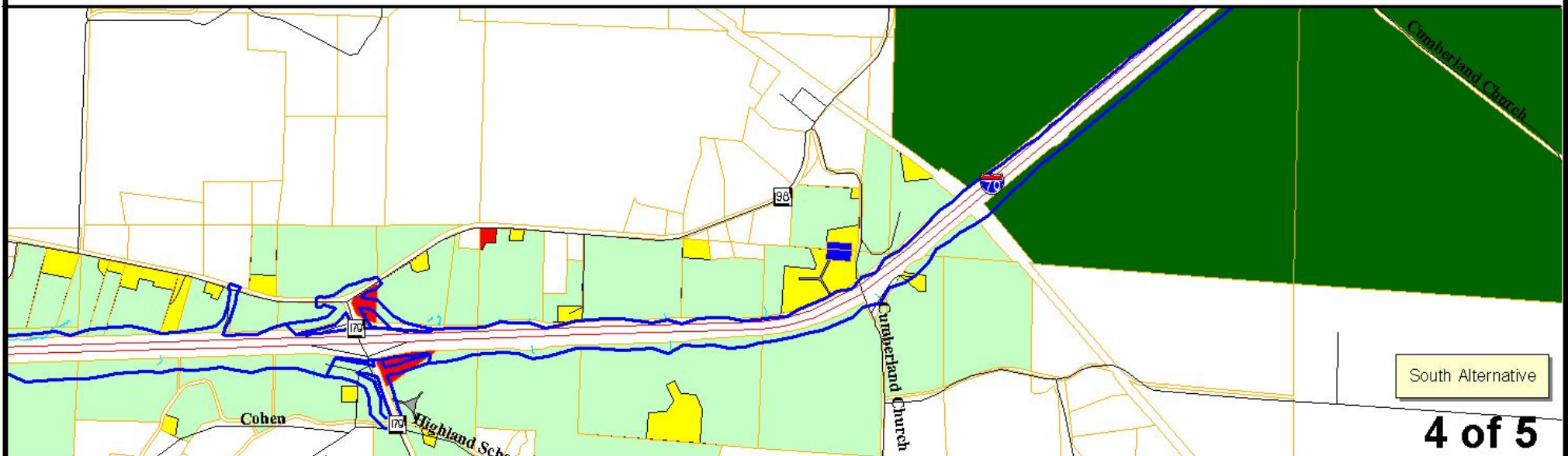
Figure III-3 Land Use Cooper & Boone Counties, Missouri
