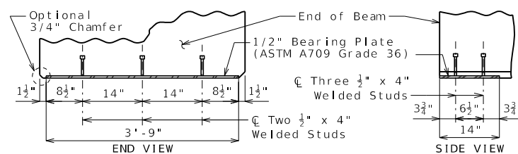
BEARING PLATE
