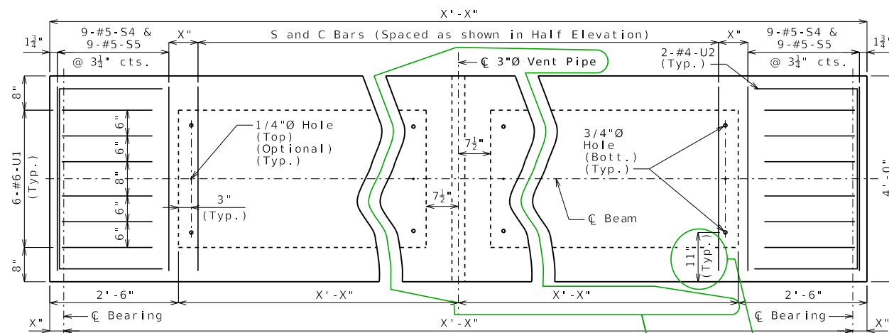
PART PLAN
