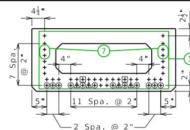
STRAND ARRANGEMENT
