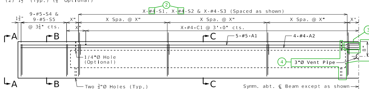
HALF ELEVATION
