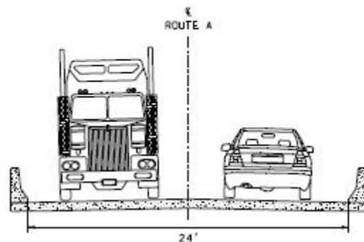
PROPOSED BRIDGE TYPICAL SECTION
