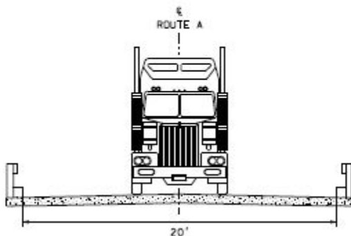
EXISTING BRIDGE TYPICAL SECTION
