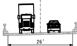
EXISTING BRIDGE TYPICAL SECTION € ROUTE 40
