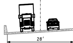
PROPOSED BRIDGE TYPICAL SECTION € ROUTE 40
