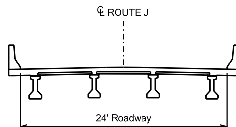
PROPOSED BRIDGE DECK ROUTE J - BRIDGE NO. A8880 ★ Proposed Bridge Deck - Construction Year 2021
