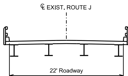
EXISTING BRIDGE DECK ROUTE J - BRIDGE NO. X0417 ★ Existing Bridge was constructed in 1938
