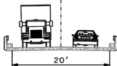
EXISTING BRIDGE TYPICAL SECTION € I-70 OUTER ROAD
