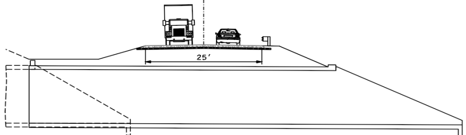
PROPOSED BOX EXTENSION TYPICAL SECTION € I-70 OUTER ROAD
