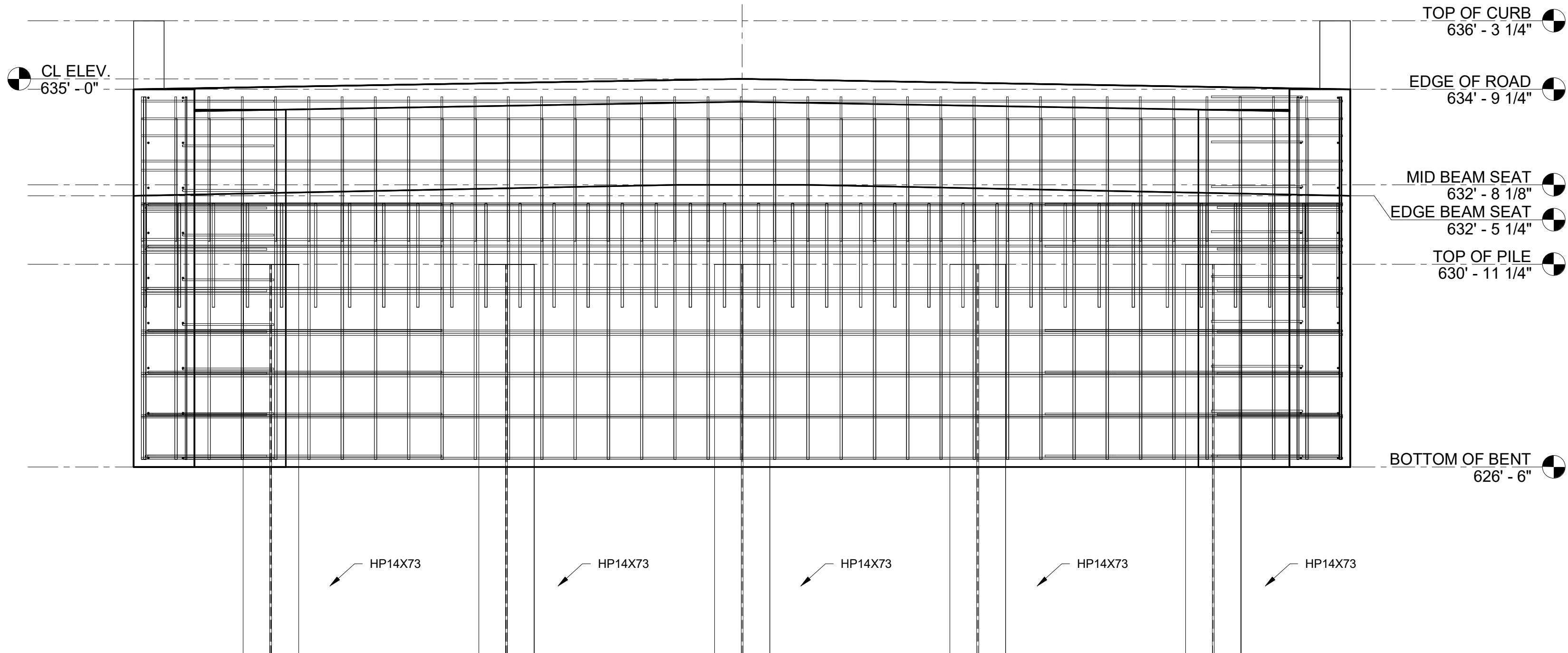
④ SOUTH ABUTMENT ELEVATION 1/2" = 1'-0"
