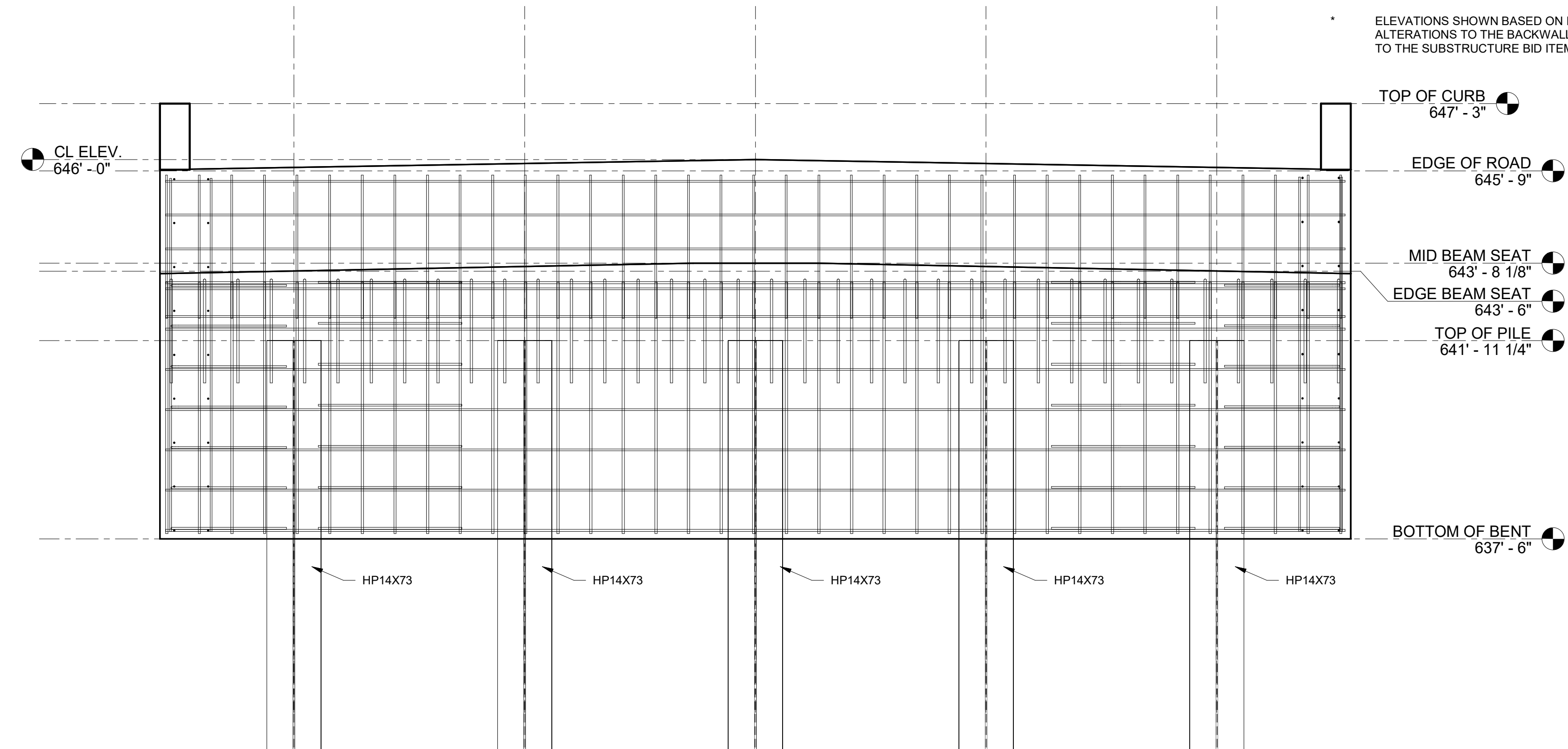
④ EAST ABUTMENT ELEVATION 1/2" = 1'-0"
