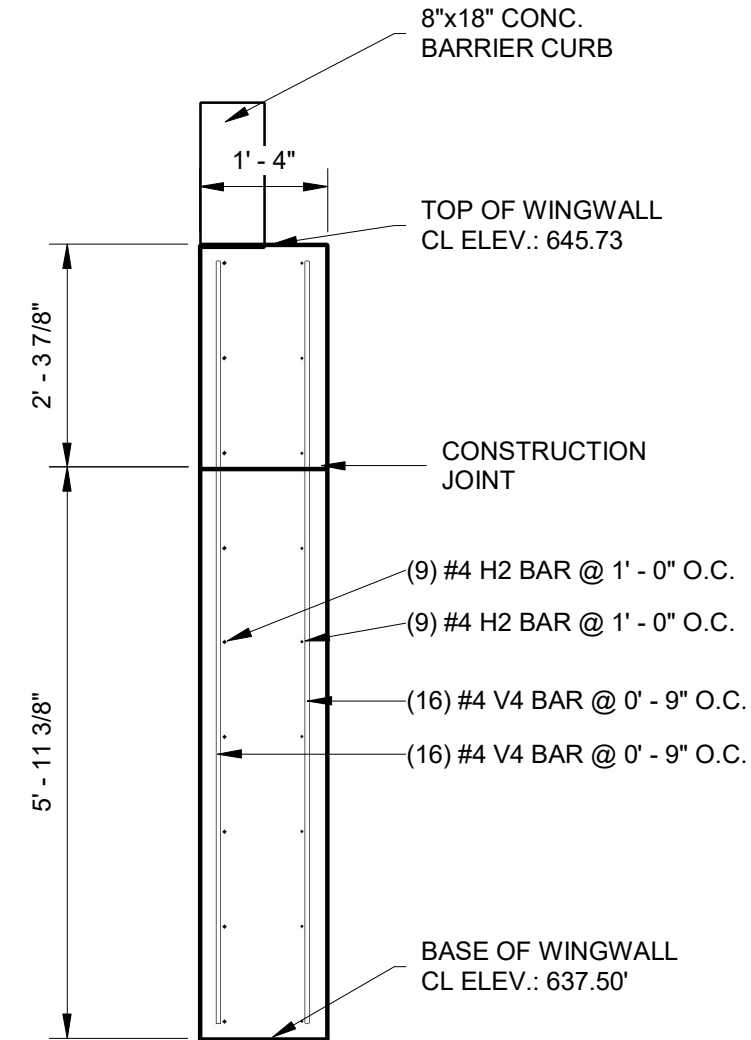
④ WEST WINGWALL SECTION 1/2" = 1'-0"
