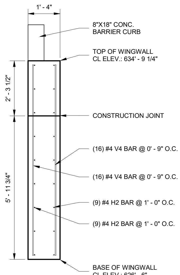
③ SOUTH WINGWALL SECTION 1/2" = 1'-0"
