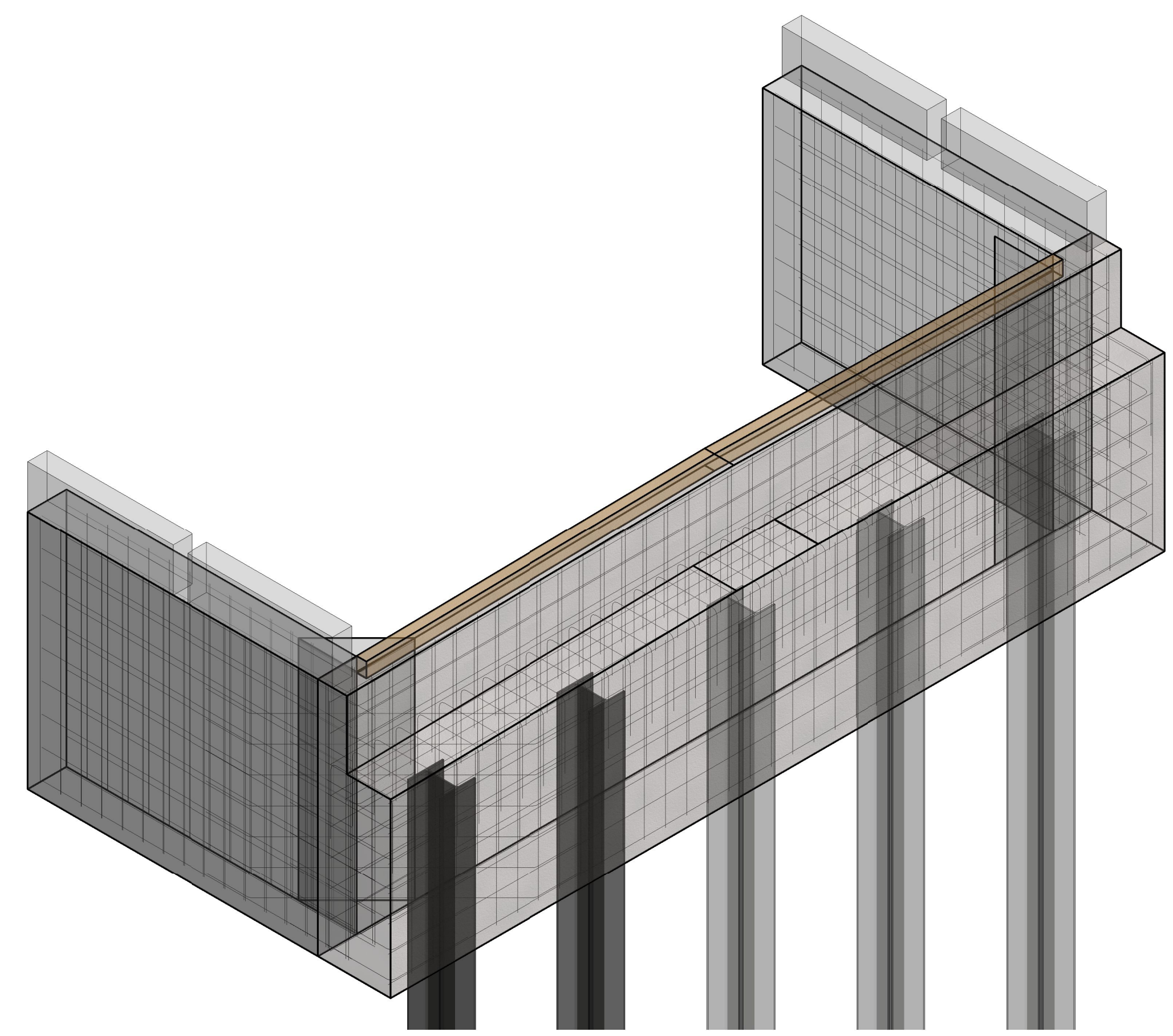
⑤ SOUTH ABUTMENT
