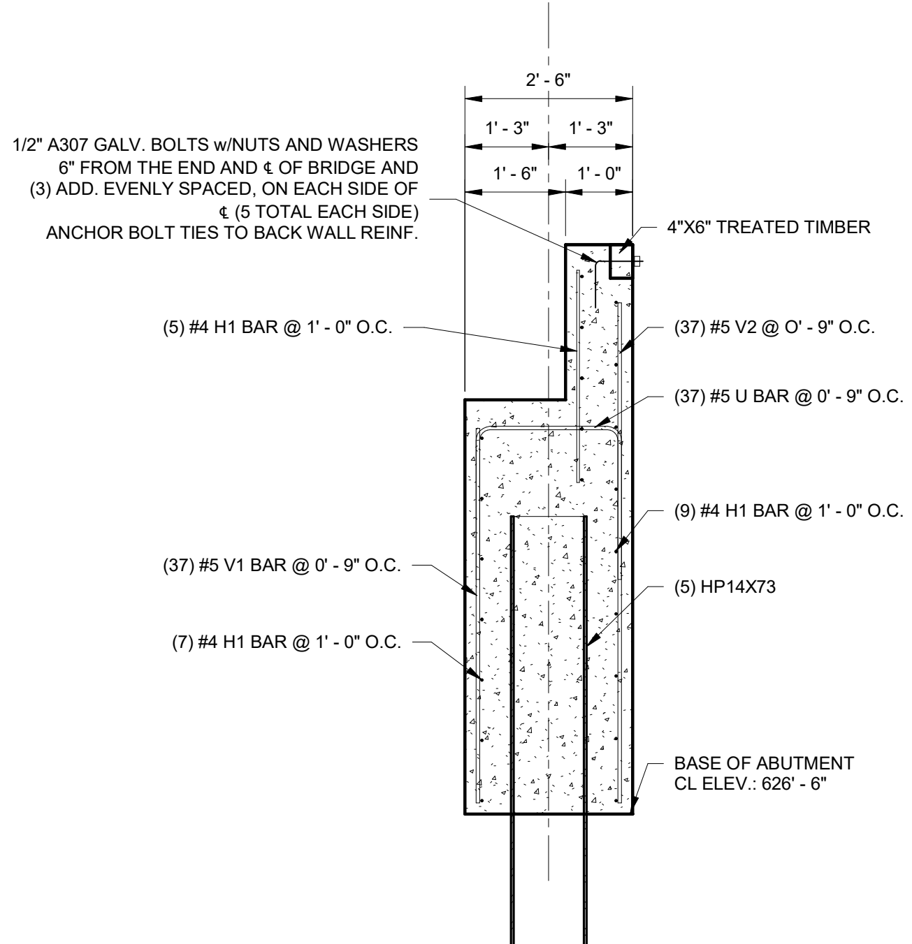
② SOUTH ABUTMENT SECTION 1/2" = 1'-0"
