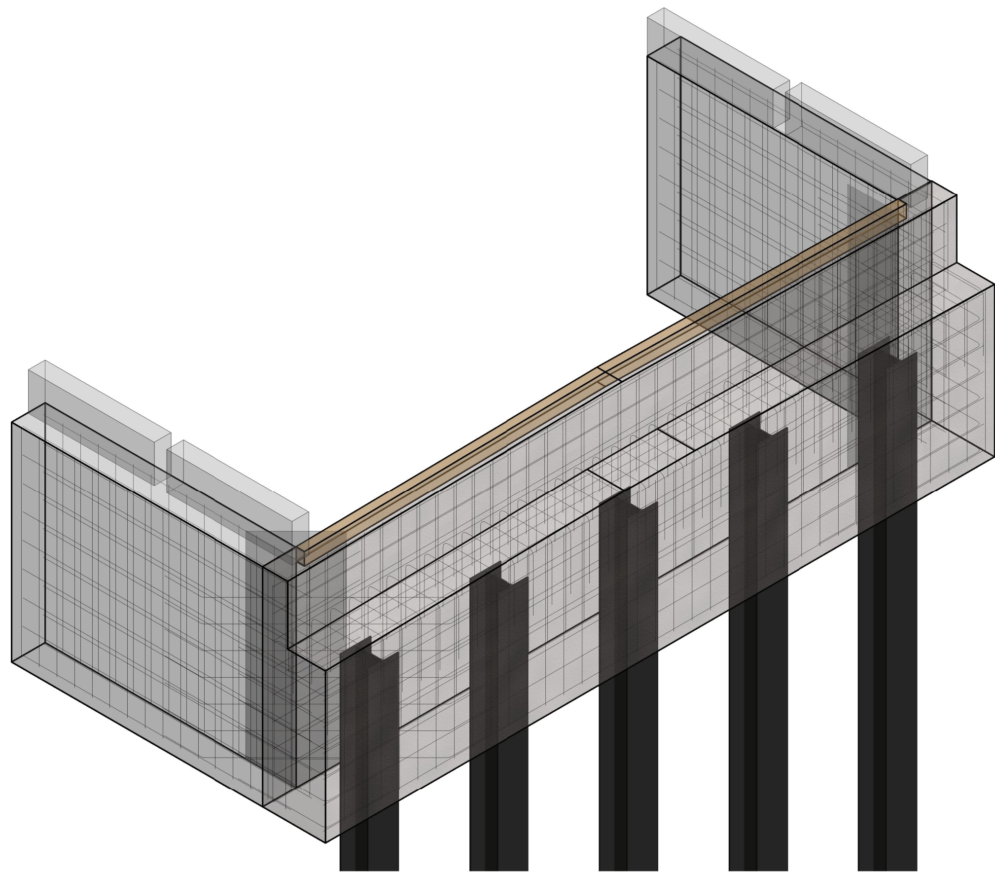
⑤ WEST ABUTMENT
