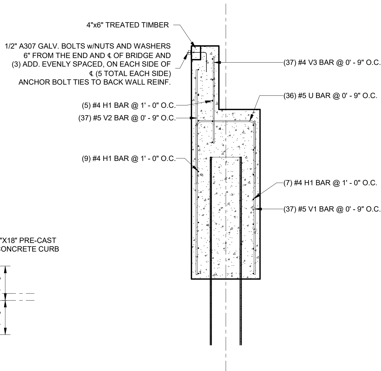
③ WEST ABUTMENT SECTION 1/2" = 1'-0"
