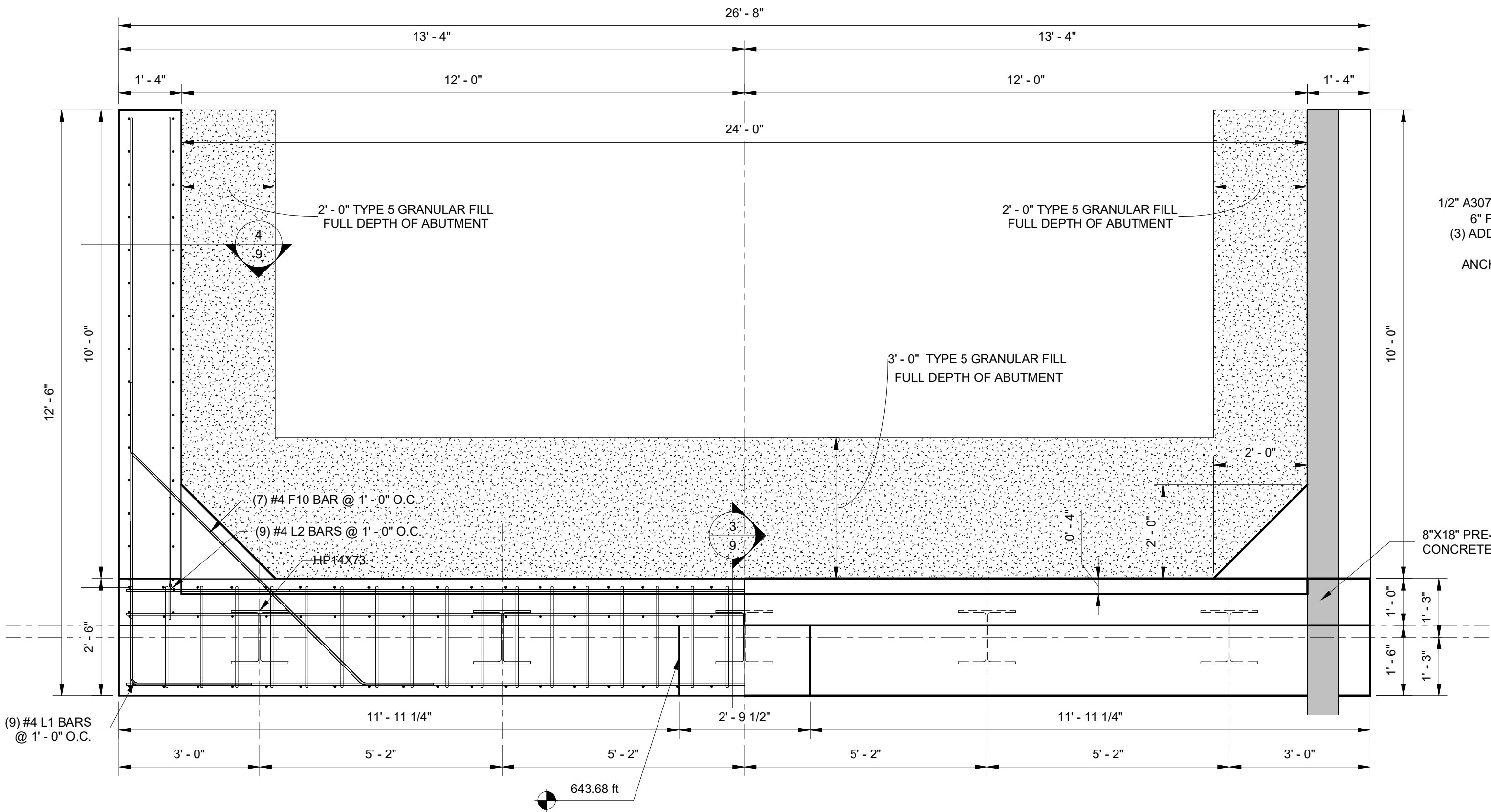
① WEST ABUTMENT PLAN VIEW 1/2" = 1'-0"
