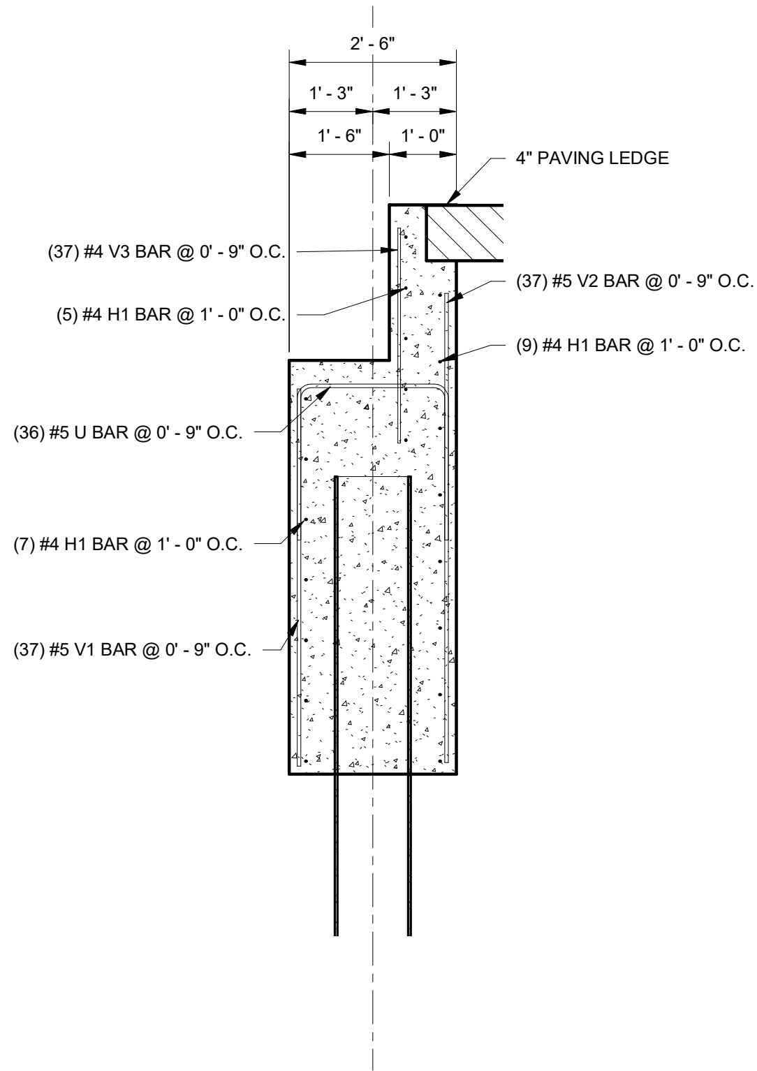
② EAST ABUTMENT SECTION 1/2" = 1'-0"
