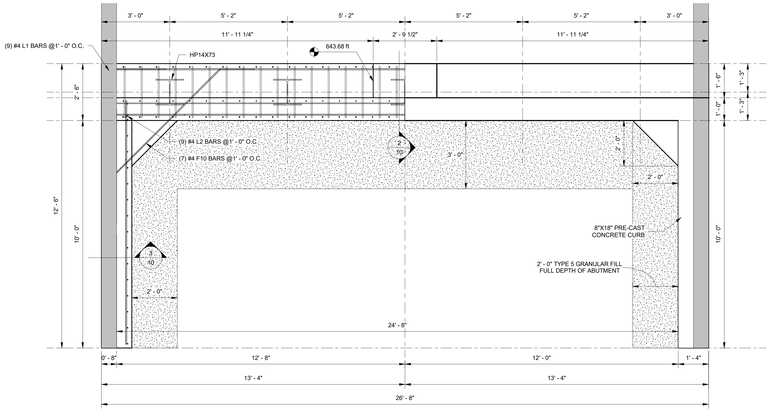
① EAST ABUTMENT PLAN VIEW 1/2" = 1'-0"
