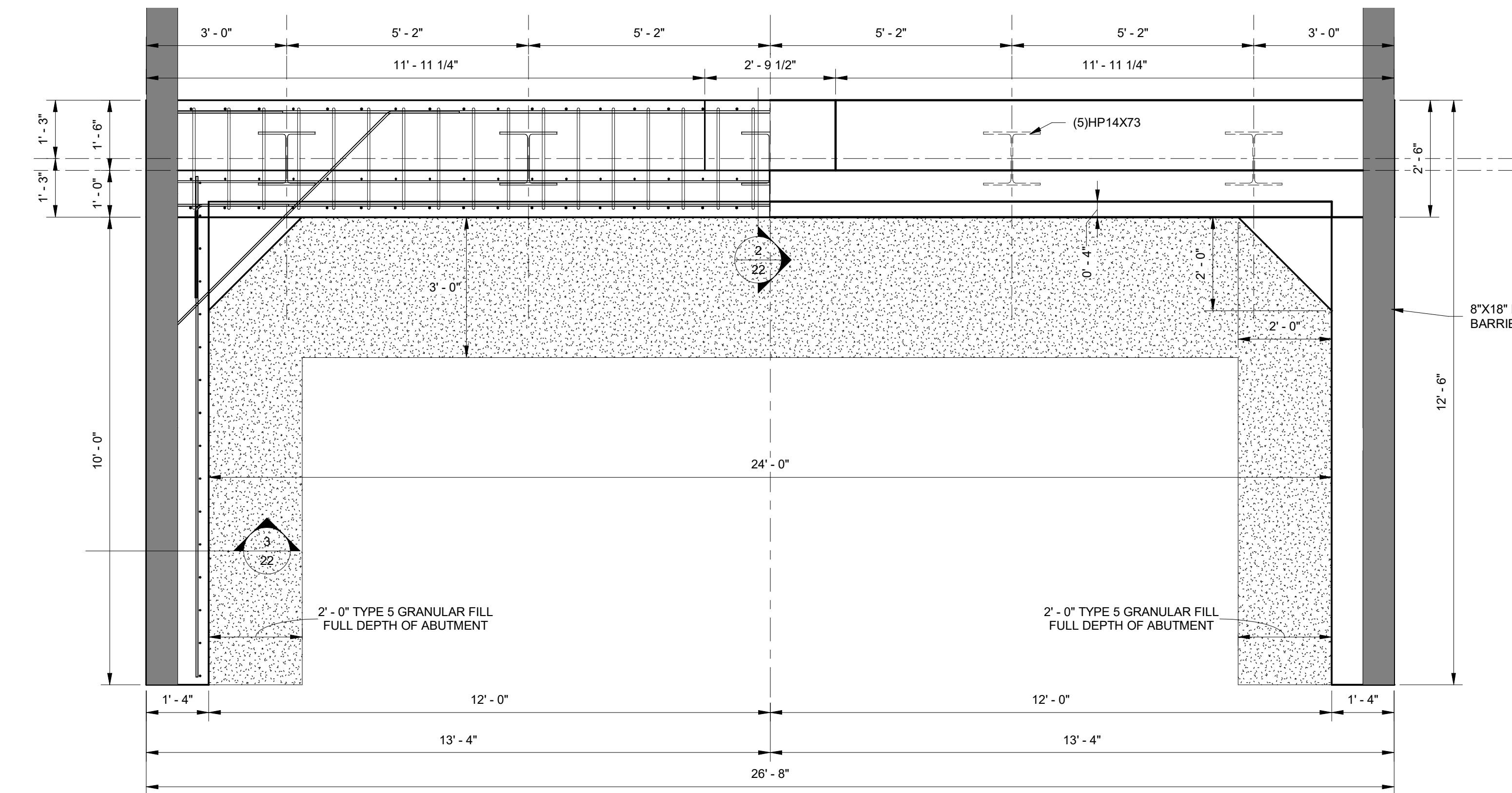
① SOUTH ABUTMENT PLAN VIEW 1/2" = 1'-0"
