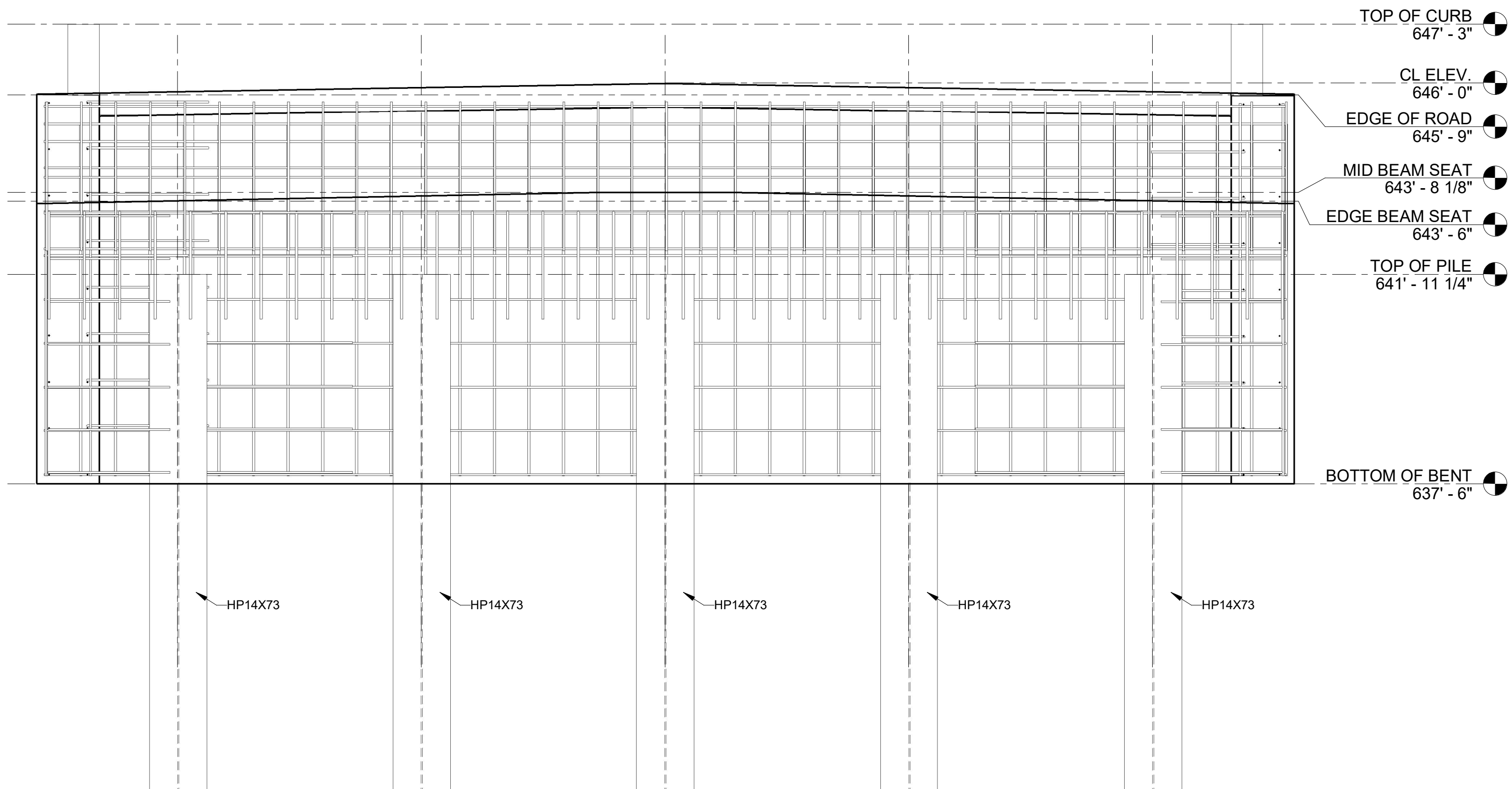
② WEST ABUTMENT ELEVATION 1/2" = 1'-0"
