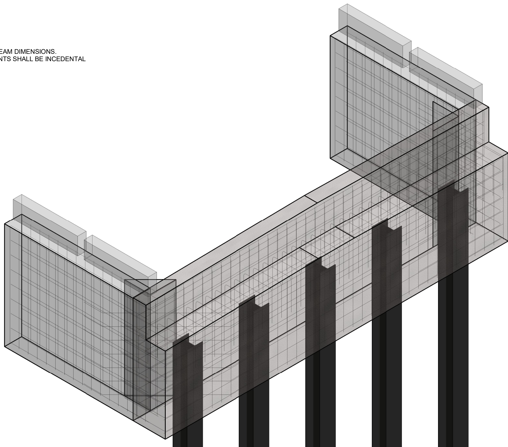
⑤ EAST ABUTMENT
