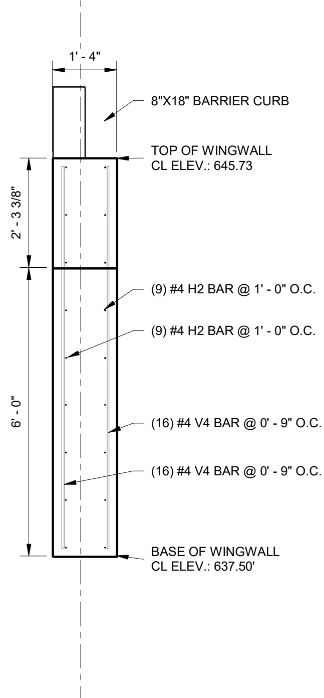
③ EAST WINGWALL SECTION 1/2" = 1'-0"
