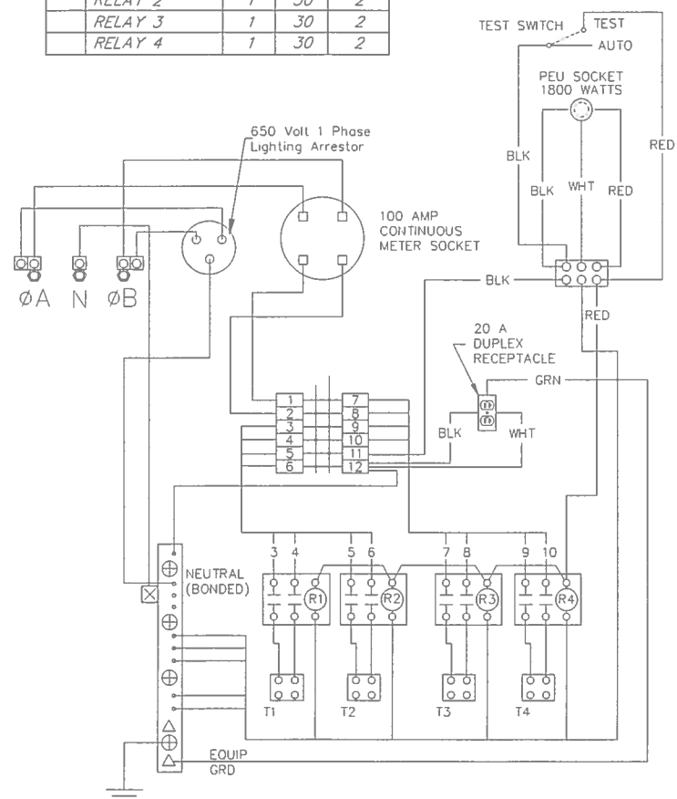
WIRING DIAGRAM
