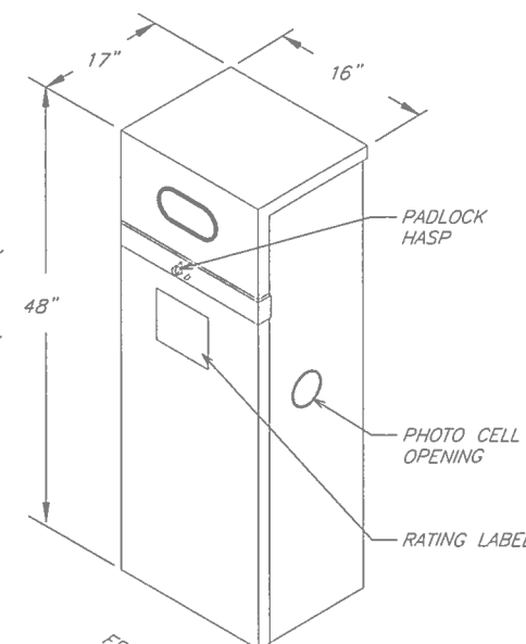
PAD MOUNTED CONTROL CENTER * FOUR-CIRCUIT CONTROLLER
