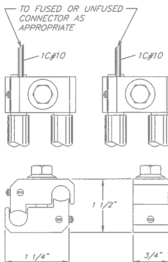
FARGO CONNECTOR
