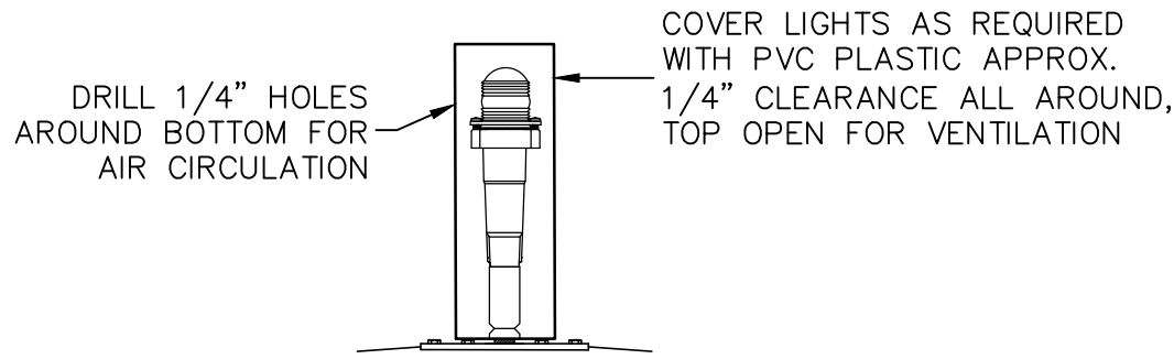
LIGHT COVER DETAIL NO SCALE
