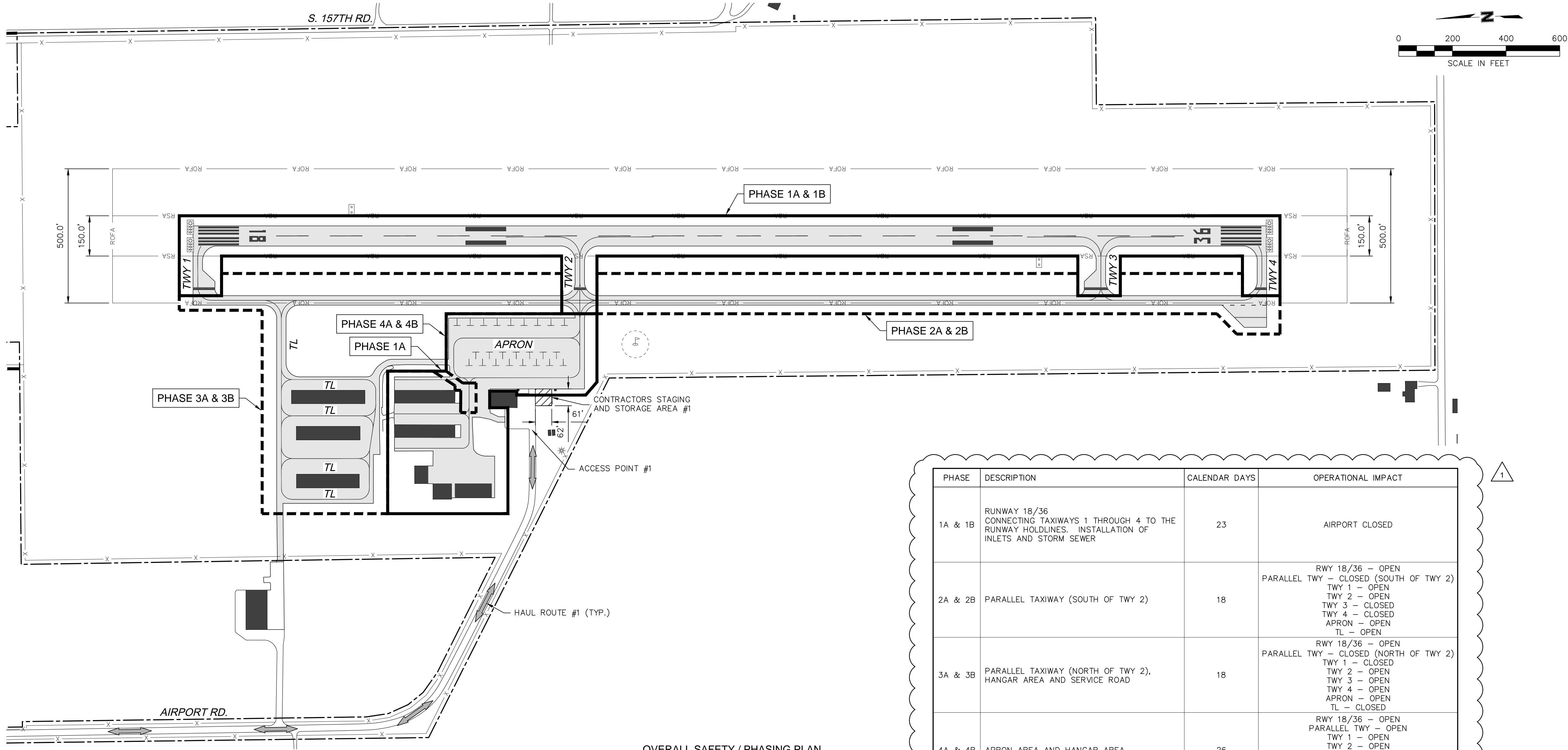
OVERALL SAFETY / PHASING PLAN
