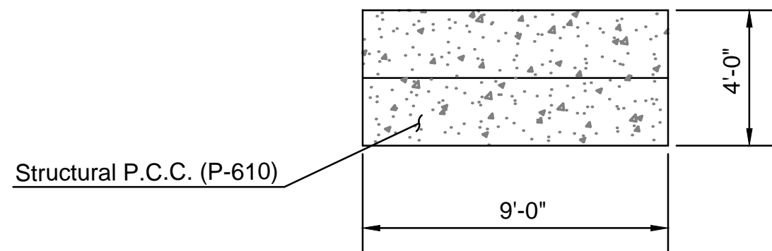
PLAN VIEW
