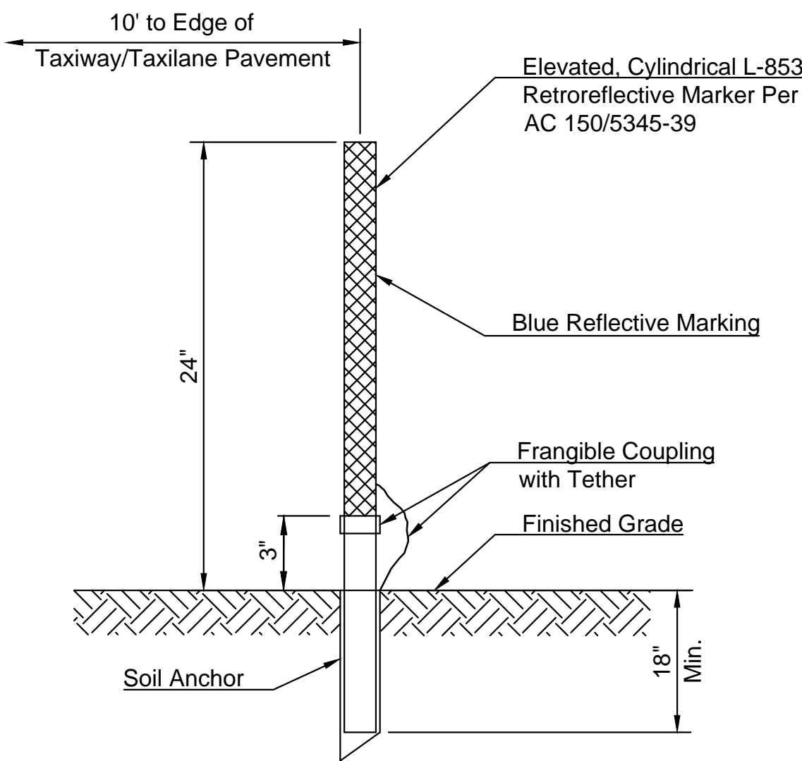
SOIL MOUNTED RETROREFLECTIVE MARKER DETAIL
