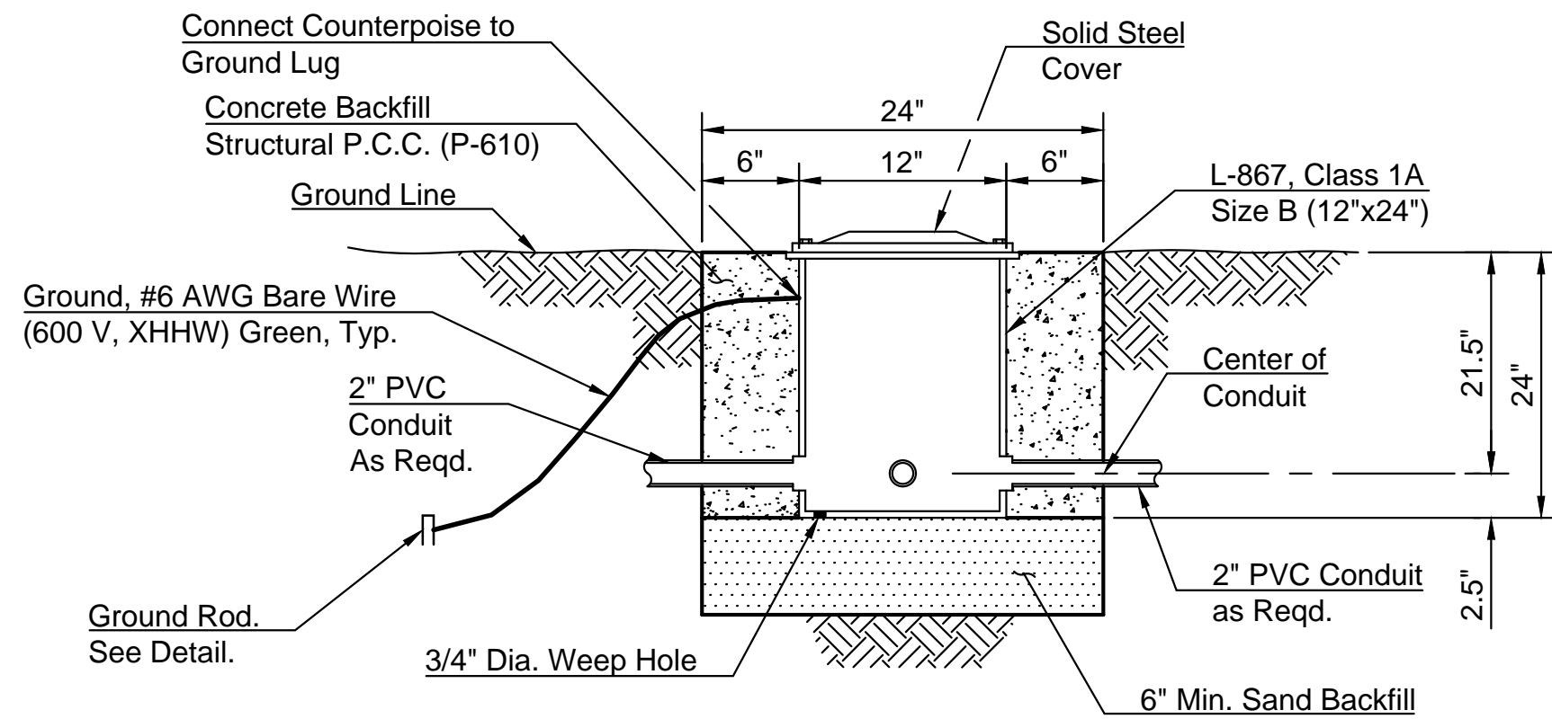
TYPICAL L-867 JUNCTION BOX
