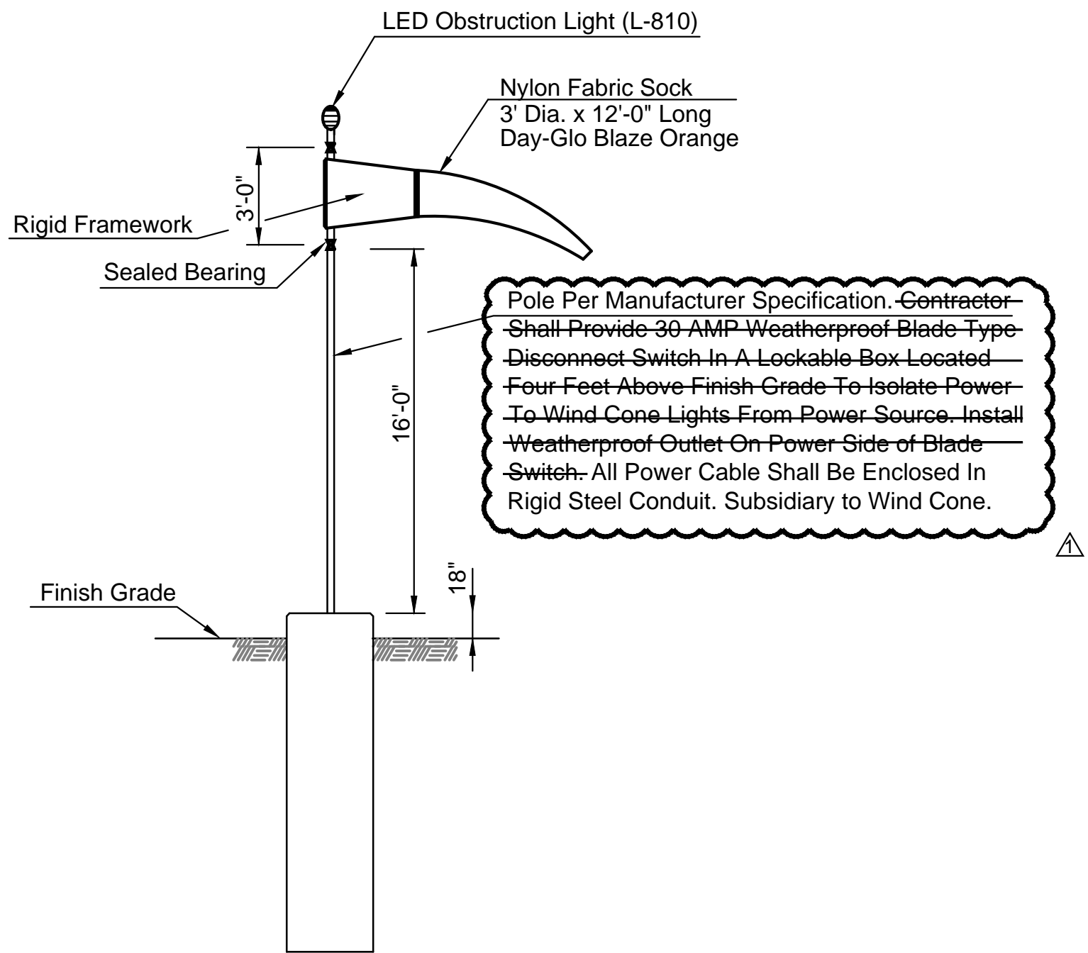
TYPE L-807 (L), STYLE I-B, SIZE 2, WIND CONE AND FOUNDATION (INTERNALLY LIGHTED WITH LED LAMPS)
