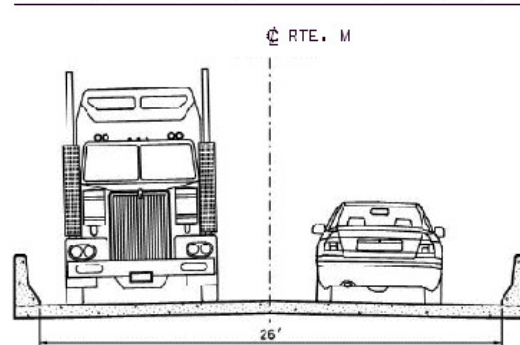
PROPOSED BRIDGE DECK
