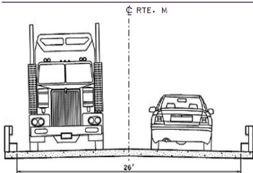
EXISTING BRIDGE DECK
