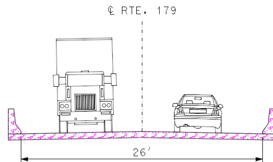
PROPOSED BRIDGE TYPICAL SECTION
