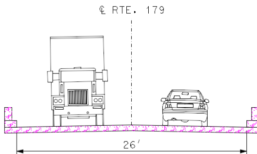
EXISTING BRIDGE TYPICAL SECTION
