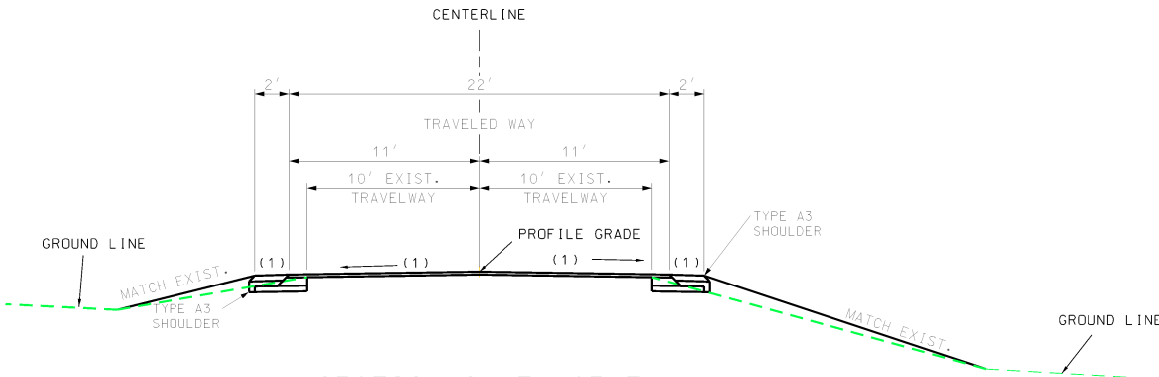
SECTION ON TANGENT TYPICAL SECTION RTE. U
