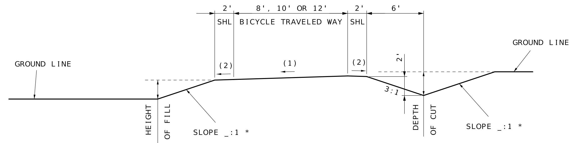
SECTION ON TANGENT TYPICAL SECTION BICYCLE PATH STA. XXX.XX TO STA. XXX.XX
