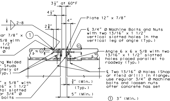
PART SECTION AT INTERMEDIATE BENT
