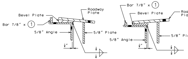
PART SECTION THRU BEVEL PLATE
