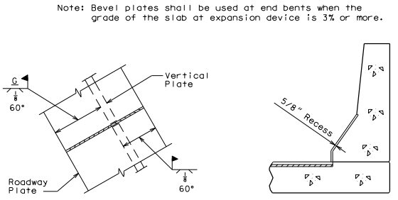
PART PLAN ROADWAY PLATE AND VERTICAL PLATE
