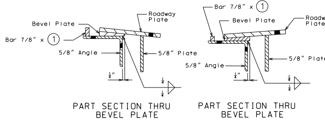
PART SECTION (TYPICAL)
