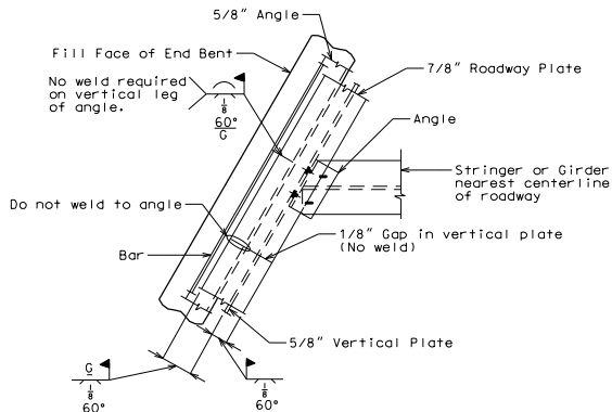
PERMISSIBLE FIELD SPICE AT END BENT
