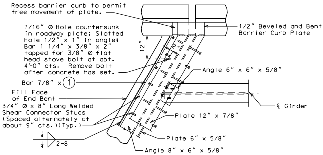
PART PLAN
