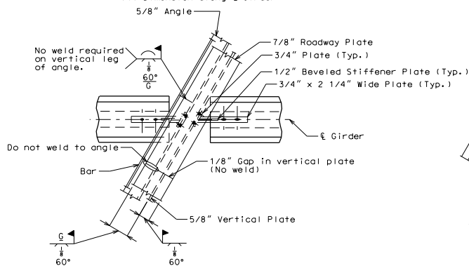
PERMISSIBLE FIELD SPLICE AT INT. BENT
