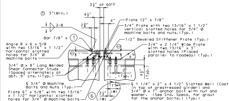
PART SECTION AT INTERMEDIATE BENT
