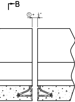
PART ELEVATION OF BARRIER CURB
