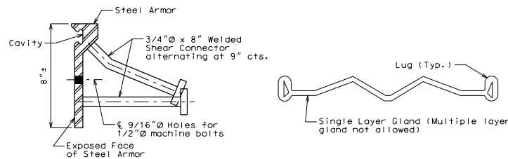
DETAIL OF JOINT ARMOR
