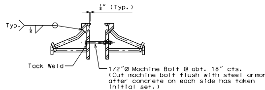
DETAIL A
