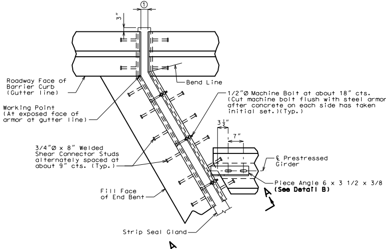
PART PLAN
