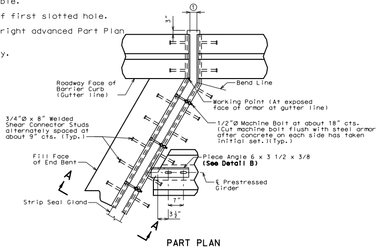
PART PLAN
