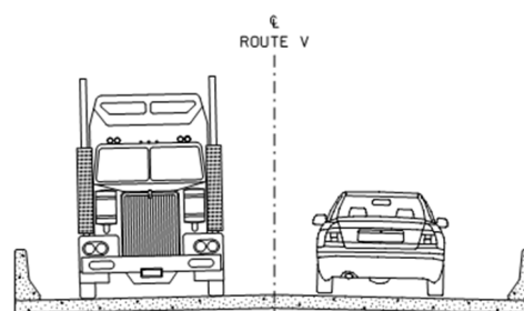
PROPOSED BRIDGE TYPICAL SECTION
