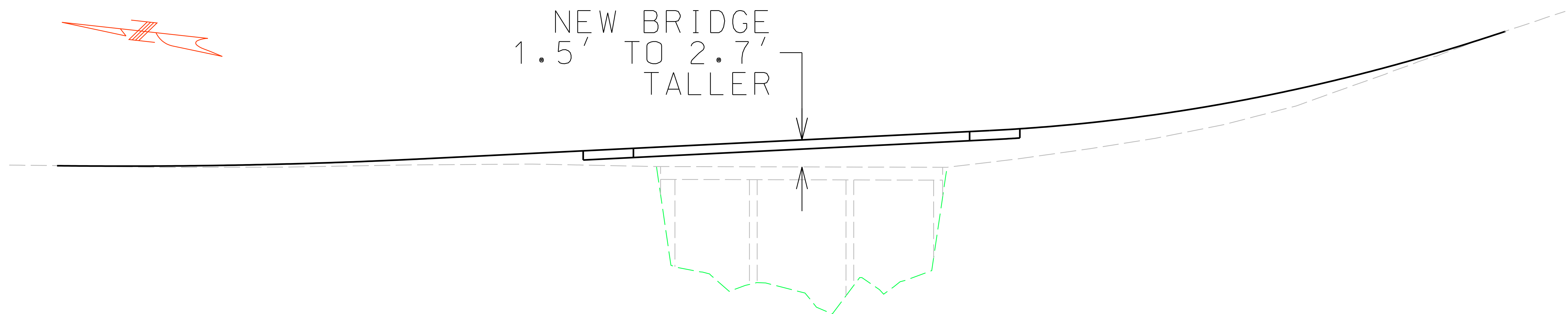
ELEVATION VIEW
