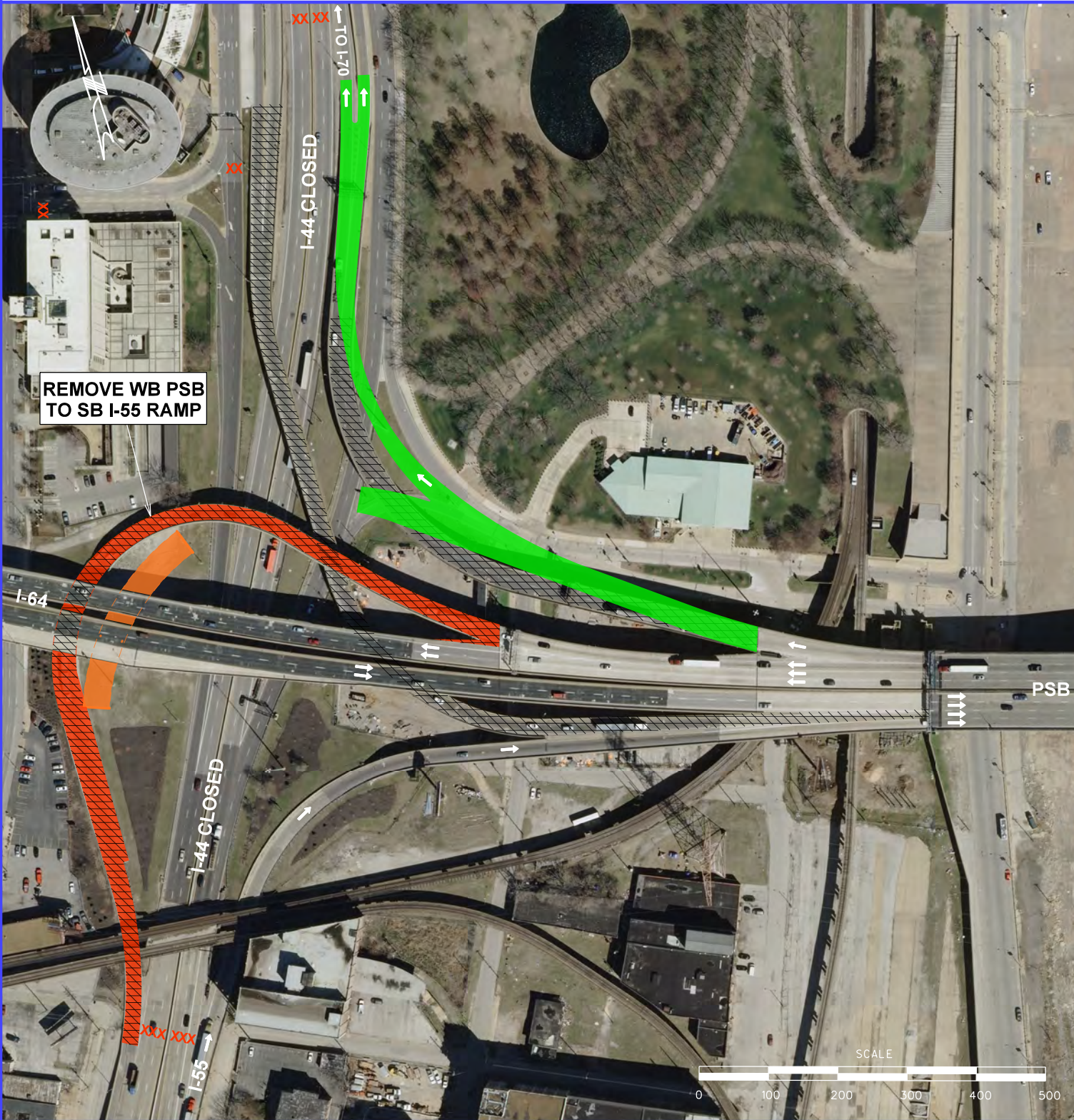
STAGING PLAN
