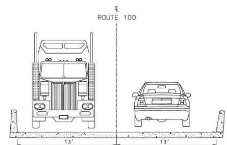
PROPOSED BRIDGE DECK ROUTE 100 - BRIDGE NO. A8890 CONSTRUCTION YEAR 2022 LENGTH = 200'
