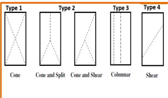
Figure 2: A Few Types of Fracture Patterns
