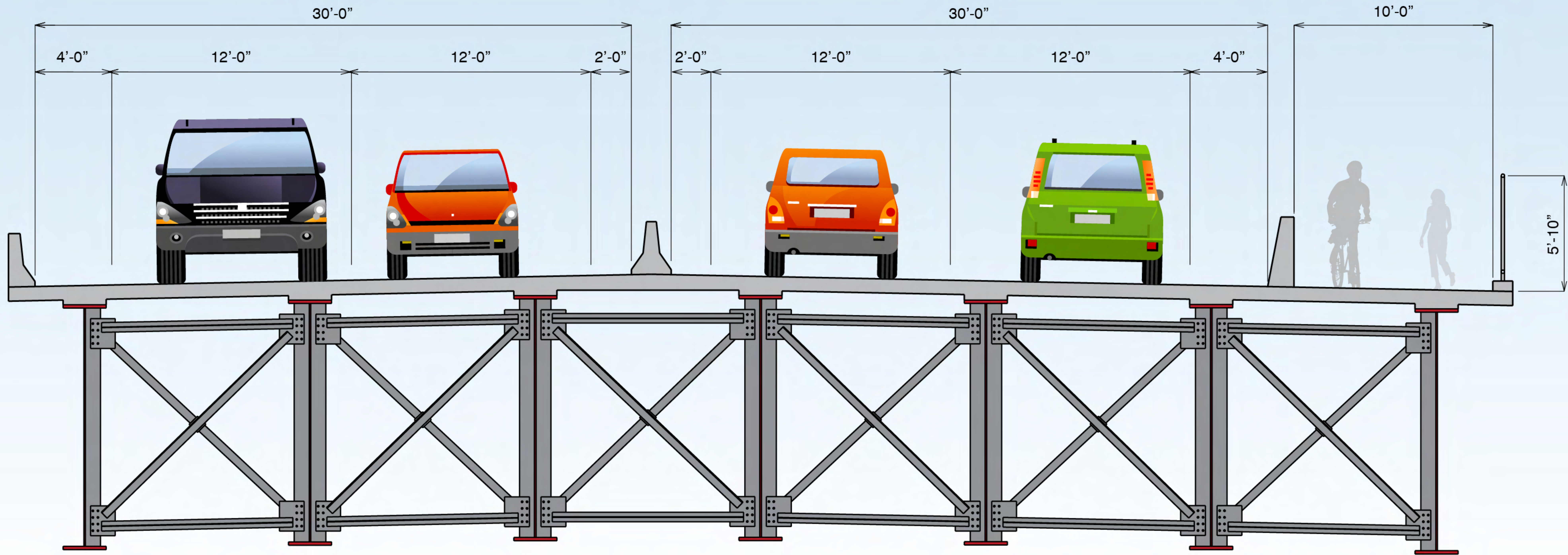
TYPICAL SECTION - UNIT 1
