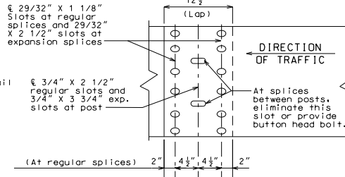
THRIE BEAM RAIL SPLICE DETAILS
