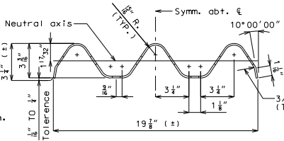
SECTION NEAR THRIE BEAM RAIL
