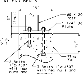
PART SECTION AT END BENT WING
