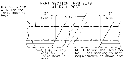
BOLTS IN GIRDER BOLTS IN DIAPHRAGM PART SECTION AT INTERMEDIATE BENT
