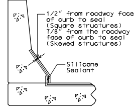
PART SECTION THRU SAFETY BARRIER CURB SHOWING SILICONE EXPANSION JOINT SEALANT
