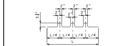
BENDING DIAGRAM FOR U1 BAR (U1 Bars may be oriented at right angles to location and spacing shown. U1 Bars shall be placed between P1 bars).
