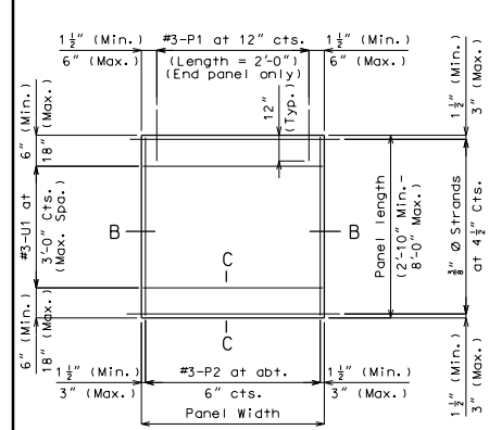
PLAN OF PRECAST PRESTRESSED PANEL
