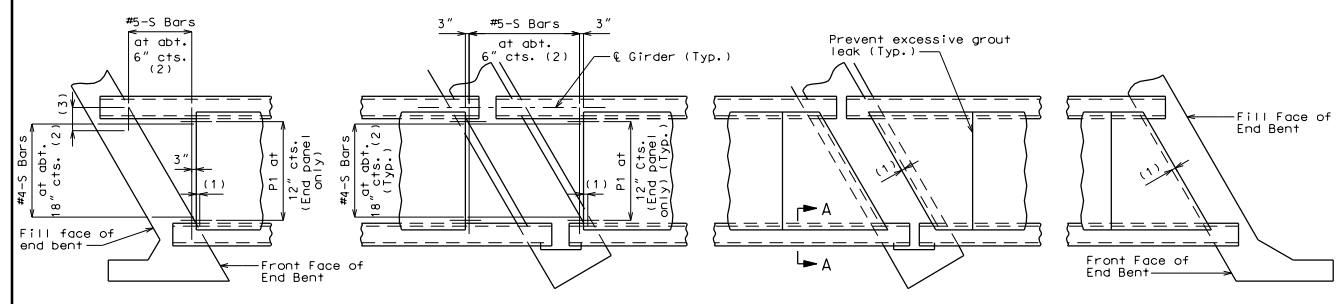
PLAN OF PRECAST PRESTRESSED PANELS PLACEMENT
