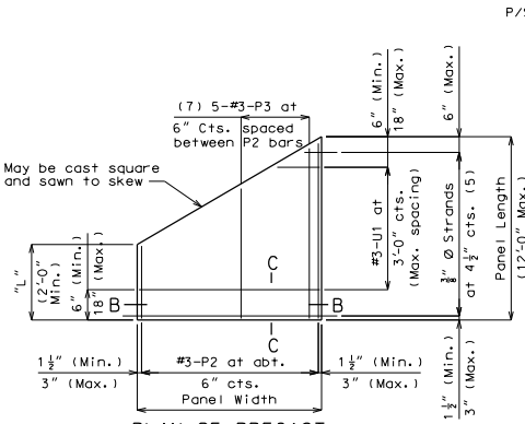
PLAN OF PRECAST PRESTRESSED PANEL (SKEWED END-OPTIONAL)
