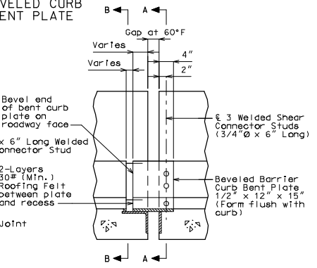
ELEVATION OF BARRIER CURB
