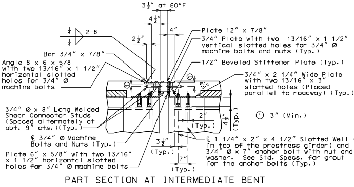
PART SECTION AT INTERMEDIATE BENT
