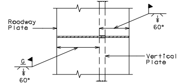
PART PLAN ROADWAY PLATE AND VERTICAL PLATE
