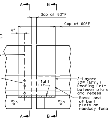
ELEVATION OF BARRIER CURB
