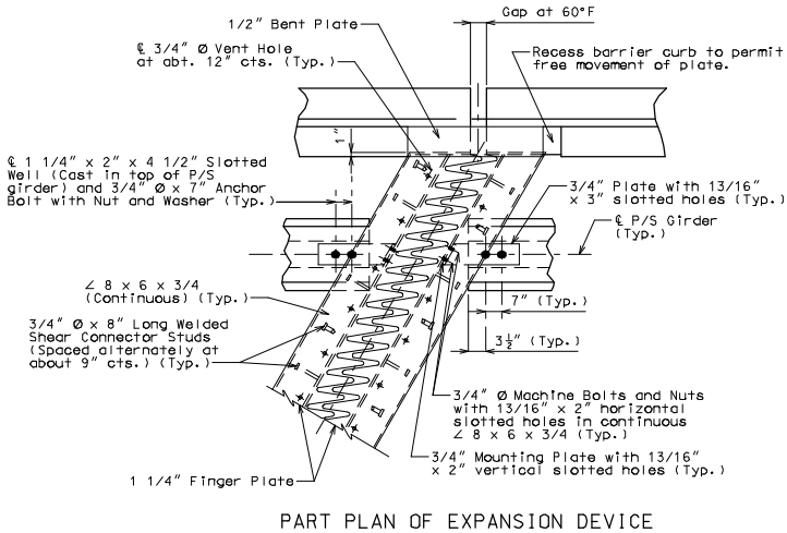
PART PLAN OF EXPANSION DEVICE
