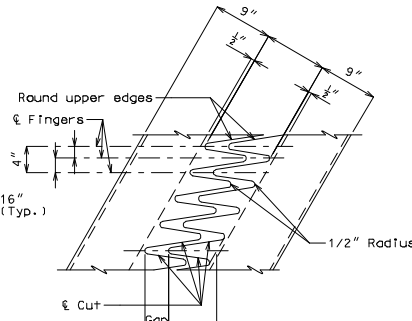
TYPICAL PLAN OF PLATE
